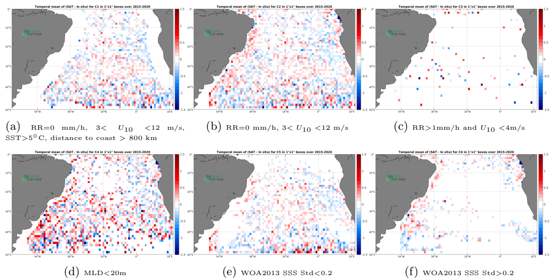
Figure 12: Temporal mean gridded over spatial boxes of size 1^\circ \times 1^\circ of \Delta SSS (SMAP SSS L2 v4 (RSS) - Argo) for 6 different subdatasets corresponding to: RR=0 mm/h, 3 < U_{10} < 12 m/s, SST > 5^\circ C , distance to coast > 800 km (a), RR=0 mm/h, 3 < U_{10} < 12 m/s (b), RR > 1 mm/h and U_{10} < 4 m/s (c), MLD < 20 m (d), WOA2013 SSS Std < 0.2 (e), WOA2013 SSS Std > 0.2 (f).
