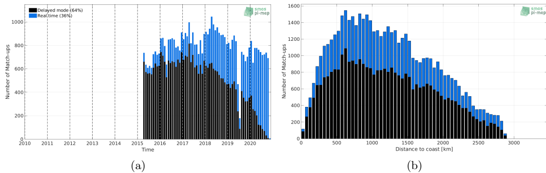
Figure 1: Number of match-ups between Argo and SMAP SSS L2 v4 (RSS) SSS as a function of time (a) and as function of the distance to coast (b) over the South Atlantic Ocean Pi-MEP region and for the full satellite product period.
