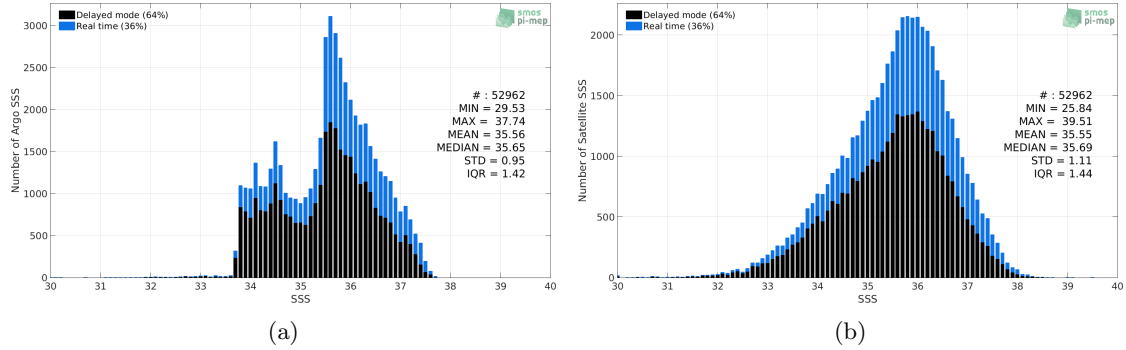
Figure 2: Histograms of SSS from Argo (a) and SMAP SSS L2 v4 (RSS) (b) considering all match-up pairs per bins of 0.1 over the South Atlantic Ocean Pi-MEP region and for the full satellite product period.
