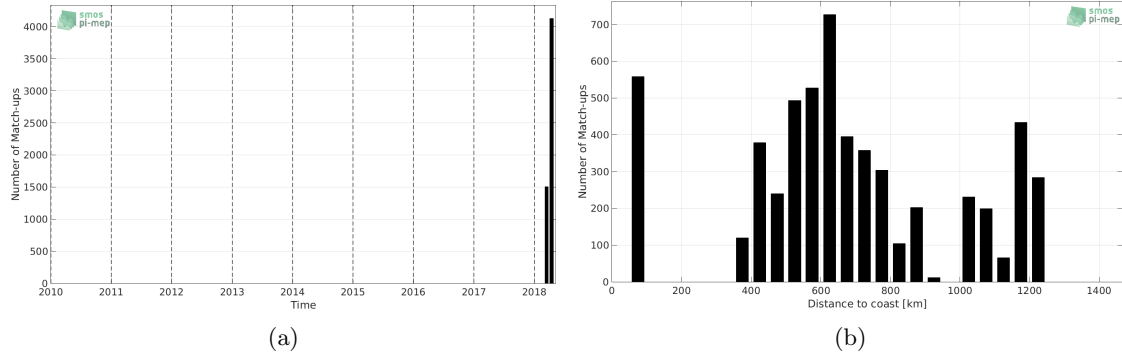
Figure 1: Number of match-ups between TSG-SAMOS and SMAP-L2-RSS-V3-70KM SSS as a function of time (a) and as function of the distance to coast (b) over the South Atlantic Ocean Pi-MEP region and for the full satellite product period.
