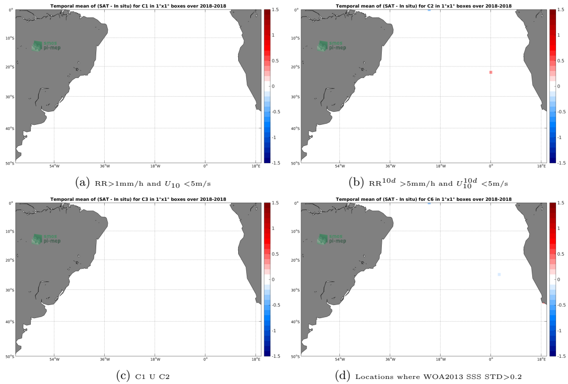
Figure 12: Temporal mean gridded over spatial boxes of size 1^\circ \times 1^\circ of \Delta SSS (SMAP-L2-RSS-V3-70KM - TSG-SAMOS) for 4 different subdatasets corresponding to: RR > 1mm/h and U_{10} < 5\text{m/s} (a), RR^{10d} > 5\text{mm/h} and U_{10}^{10d} < 5\text{m/s} (b), C1 U C2 (c), Locations where WOA2013 SSS STD > 0.2 (d).
