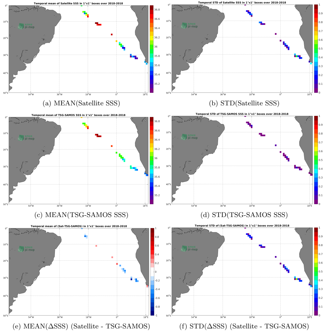
Figure 6: Temporal mean (left) and STD (right) of SSS from SMAP-L2-RSS-V3-70KM (top), TSG-SAMOS (middle), and of \Delta SSS (Satellite - TSG-SAMOS). Only match-up pairs are used to generate these maps.
