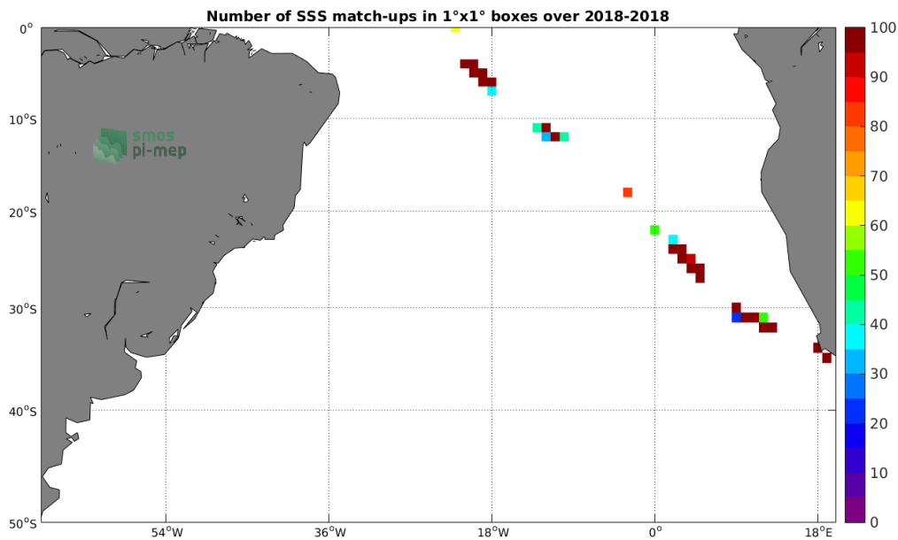
Figure 4: Number of SSS match-ups between TSG-SAMOS SSS and the SMAP-L2-RSS-V3-70KM SSS product for the South Atlantic Ocean Pi-MEP region over 1^\circ \times 1^\circ boxes and for the full satellite product period.
