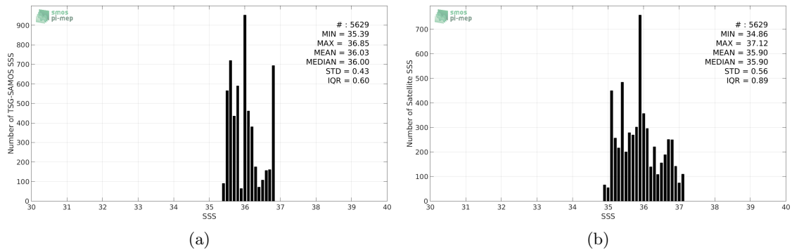
Figure 2: Histograms of SSS from TSG-SAMOS (a) and SMAP-L2-RSS-V3-70KM (b) considering all match-up pairs per bins of 0.1 over the South Atlantic Ocean Pi-MEP region and for the full satellite product period.
