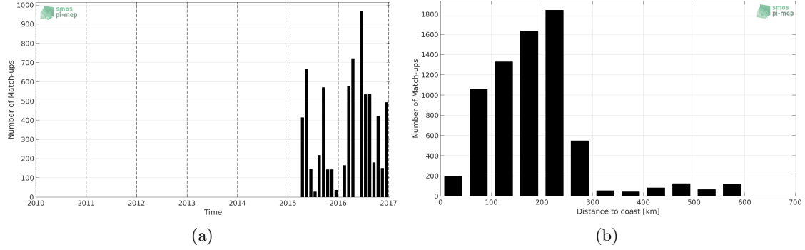
Figure 1: Number of match-ups between TSG-LEGOS-DM and SMAP-L2-RSS-V3-70KM SSS as a function of time (a) and as function of the distance to coast (b) over the South Atlantic Ocean Pi-MEP region and for the full satellite product period.
