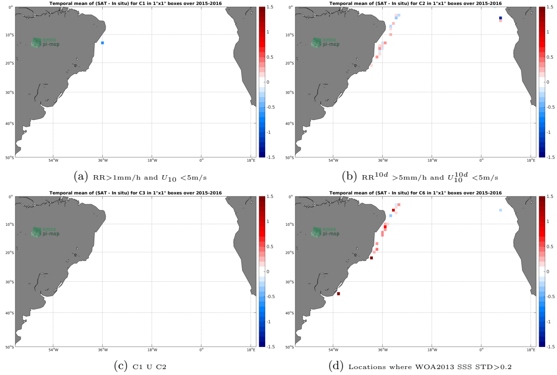
Figure 12: Temporal mean gridded over spatial boxes of size 1^\circ \times 1^\circ of \Delta SSS (SMAP-L2-RSS-V3-70KM - TSG-LEGOS-DM) for 4 different subdatasets corresponding to: RR > 1\text{mm/h} and U_{10} < 5\text{m/s} (a), RR^{10d} > 5\text{mm/h} and U_{10}^{10d} < 5\text{m/s} (b), C1 U C2 (c), Locations where WOA2013 SSS STD > 0.2 (d).
