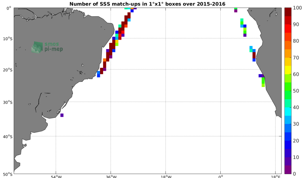
Figure 4: Number of SSS match-ups between TSG-LEGOS-DM SSS and the SMAP-L2-RSS-V3-70KM SSS product for the South Atlantic Ocean Pi-MEP region over 1^\circ \times 1^\circ boxes and for the full satellite product period.
