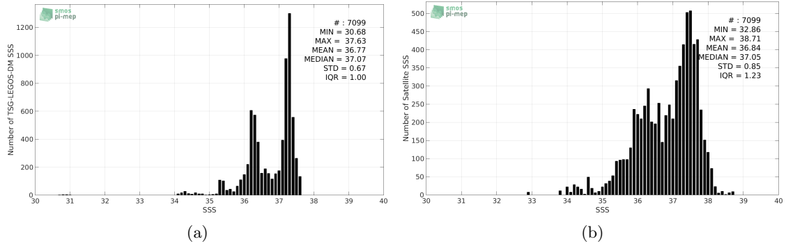
Figure 2: Histograms of SSS from TSG-LEGOS-DM (a) and SMAP-L2-RSS-V3-70KM (b) considering all match-up pairs per bins of 0.1 over the South Atlantic Ocean Pi-MEP region and for the full satellite product period.
