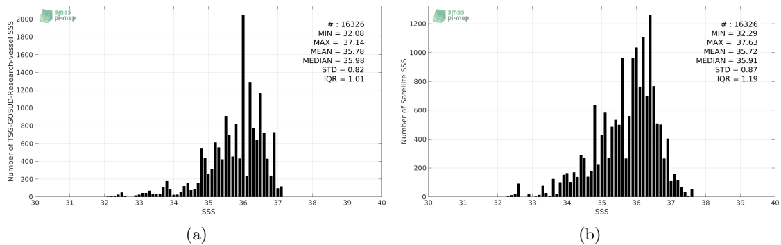
Figure 2: Histograms of SSS from TSG-GOSUD-Research-vessel (a) and SMAP-L2-RSS-V3-70KM (b) considering all match-up pairs per bins of 0.1 over the South Atlantic Ocean Pi-MEP region and for the full satellite product period.
