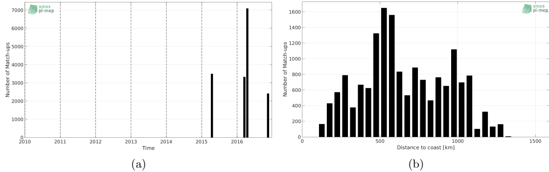
Figure 1: Number of match-ups between TSG-GOSUD-Research-vessel and SMAP-L2-RSS-V3-70KM SSS as a function of time (a) and as function of the distance to coast (b) over the South Atlantic Ocean Pi-MEP region and for the full satellite product period.
