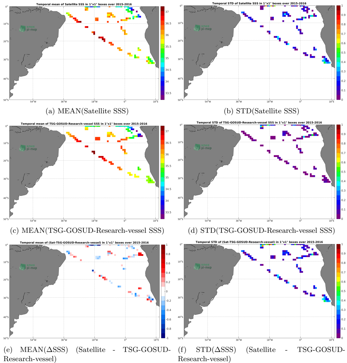
Figure 6: Temporal mean (left) and STD (right) of SSS from SMAP-L2-RSS-V3-70KM (top), TSG-GOSUD-Research-vessel (middle), and of \Delta SSS (Satellite - TSG-GOSUD-Research-vessel). Only match-up pairs are used to generate these maps.
