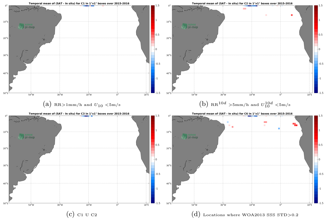
Figure 12: Temporal mean gridded over spatial boxes of size 1^\circ \times 1^\circ of \Delta SSS (SMAP-L2-RSS-V3-70KM - TSG-GOSUD-Research-vessel) for 4 different subdatasets corresponding to: RR > 1mm/h and U_{10} < 5\text{m/s} (a), RR^{10d} > 5\text{mm/h} and U_{10}^{10d} < 5\text{m/s} (b), C1 U C2 (c), Locations where WOA2013 SSS STD > 0.2 (d).
