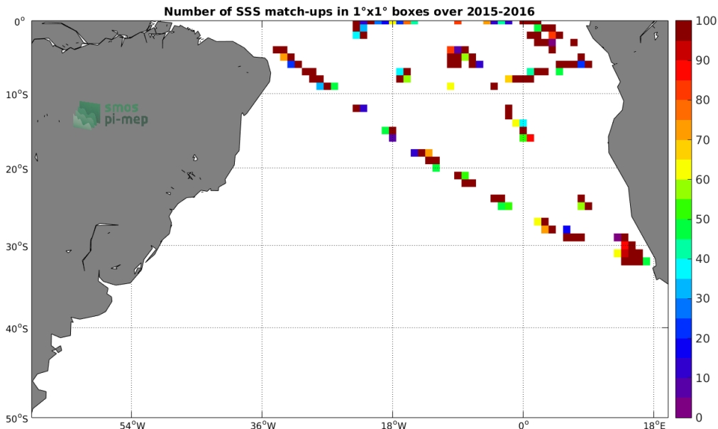
Figure 4: Number of SSS match-ups between TSG-GOSUD-Research-vessel SSS and the SMAP-L2-RSS-V3-70KM SSS product for the South Atlantic Ocean Pi-MEP region over 1^\circ \times 1^\circ boxes and for the full satellite product period.
