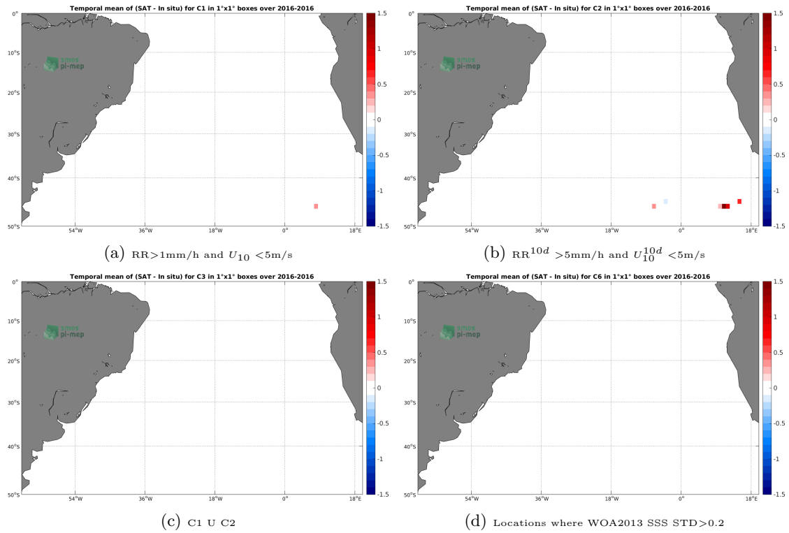
Figure 11: Temporal mean gridded over spatial boxes of size 1^\circ \times 1^\circ of \Delta SSS (SMAP-L2-RSS-V3-70KM - Surface drifters) for 4 different subdatasets corresponding to: RR > 1mm/h and U_{10} < 5\text{m/s} (a), RR^{10d} > 5\text{mm/h} and U_{10}^{10d} < 5\text{m/s} (b), C1 U C2 (c), Locations where WOA2013 SSS STD > 0.2 (d).
