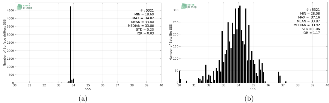
Figure 2: Histograms of SSS from Surface drifters (a) and SMAP-L2-RSS-V3-70KM (b) considering all match-up pairs per bins of 0.1 over the South Atlantic Ocean Pi-MEP region and for the full satellite product period.
