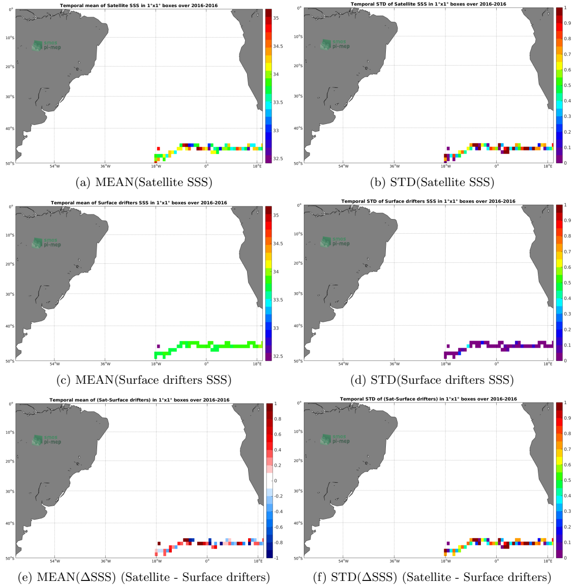
Figure 5: Temporal mean (left) and STD (right) of SSS from SMAP-L2-RSS-V3-70KM (top), Surface drifters (middle), and of \Delta\text{SSS} (Satellite - Surface drifters). Only match-up pairs are used to generate these maps.
