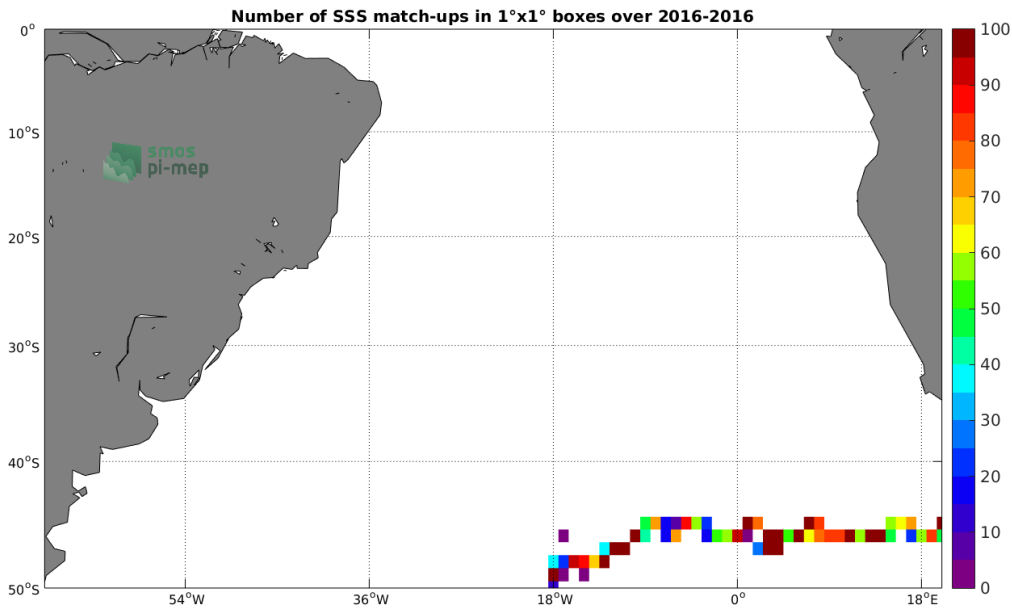
Figure 3: Number of SSS match-ups between Surface drifters SSS and the SMAP-L2-RSS-V3-70KM SSS product for the South Atlantic Ocean Pi-MEP region over 1^\circ \times 1^\circ boxes and for the full satellite product period.
