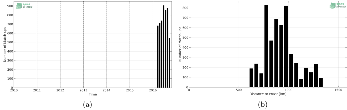
Figure 1: Number of match-ups between Surface drifters and SMAP-L2-RSS-V3-70KM SSS as a function of time (a) and as function of the distance to coast (b) over the South Atlantic Ocean Pi-MEP region and for the full satellite product period.
