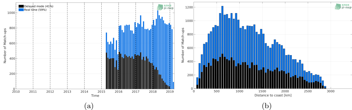
Figure 1: Number of match-ups between Argo and SMAP-L2-RSS-V3-70KM SSS as a function of time (a) and as function of the distance to coast (b) over the South Atlantic Ocean Pi-MEP region and for the full satellite product period.
