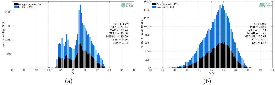
Figure 2: Histograms of SSS from Argo (a) and SMAP-L2-RSS-V3-70KM (b) considering all match-up pairs per bins of 0.1 over the South Atlantic Ocean Pi-MEP region and for the full satellite product period.
