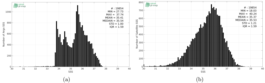
Figure 2: Histograms of SSS from Argos (a) and SMAP-L2-RSS-V3-70KM (b) considering all match-up pairs per bins of 0.1 over the South Atlantic Ocean Pi-MEP region and for the full satellite product period.
