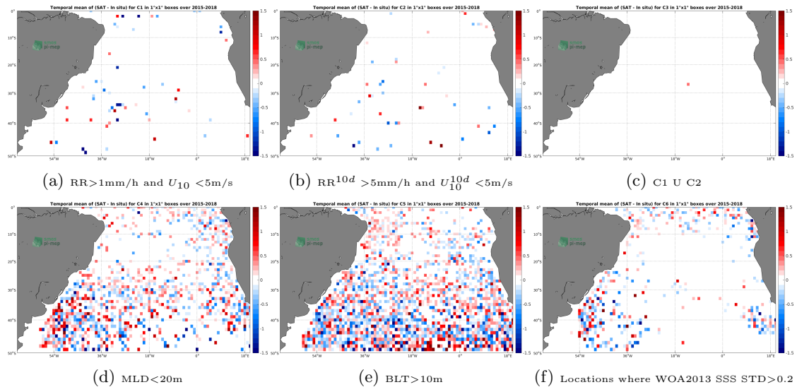
Figure 12: Temporal mean gridded over spatial boxes of size 1^\circ \times 1^\circ of \Delta\text{SSS} (SMAP-L2-RSS-V3-70KM - Argo) for 6 different subdatasets corresponding to: \text{RR} > 1\text{mm/h} and U_{10} < 5\text{m/s} (a), \text{RR}^{10d} > 5\text{mm/h} and U_{10}^{10d} < 5\text{m/s} (b), C1 U C2 (c), \text{MLD} < 20\text{m} (d), \text{BLT} > 10\text{m} (e), Locations where WOA2013 SSS STD > 0.2 (f).
