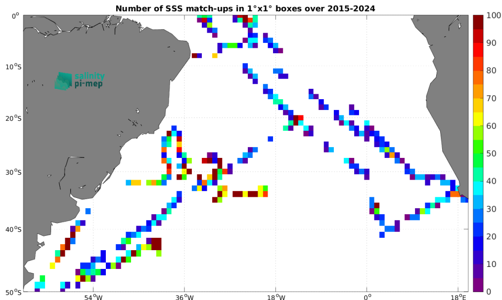
Figure 5: Number of SSS match-ups between TSG (SAMOS) SSS and the SMAP SSS L2 v5.0 (JPL) SSS product for the South Atlantic Ocean Pi-MEP region over 1^\circ \times 1^\circ boxes and for the full satellite product period.
