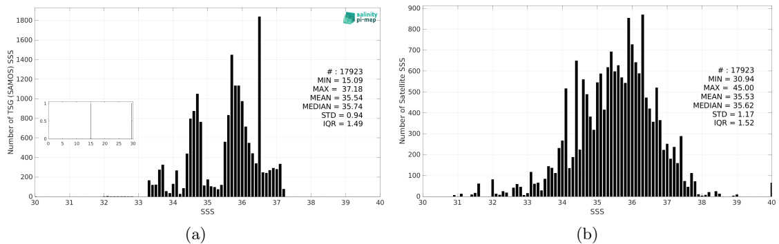
Figure 3: Histograms of SSS from TSG (SAMOS) (a) and SMAP SSS L2 v5.0 (JPL) (b) considering all match-up pairs per bins of 0.1 over the South Atlantic Ocean Pi-MEP region and for the full satellite product period.
