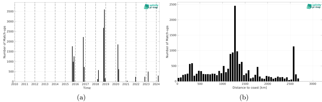
Figure 2: Number of match-ups between TSG (SAMOS) and SMAP SSS L2 v5.0 (JPL) SSS as a function of time (a) and as function of the distance to coast (b) over the South Atlantic Ocean Pi-MEP region and for the full satellite product period.
