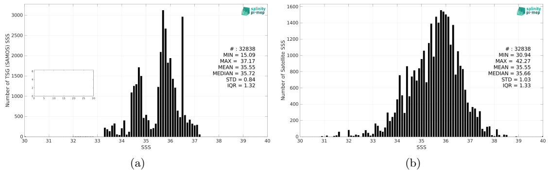
Figure 2: Histograms of SSS from TSG (SAMOS) (a) and SMAP SSS L2 v5.0 (JPL) (b) considering all match-up pairs per bins of 0.1 over the South Atlantic Ocean Pi-MEP region and for the full satellite product period.
