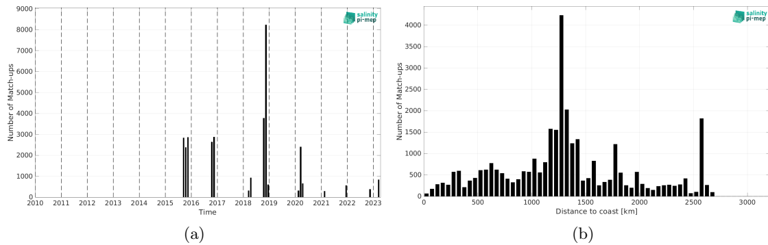
Figure 1: Number of match-ups between TSG (SAMOS) and SMAP SSS L2 v5.0 (JPL) SSS as a function of time (a) and as function of the distance to coast (b) over the South Atlantic Ocean Pi-MEP region and for the full satellite product period.
