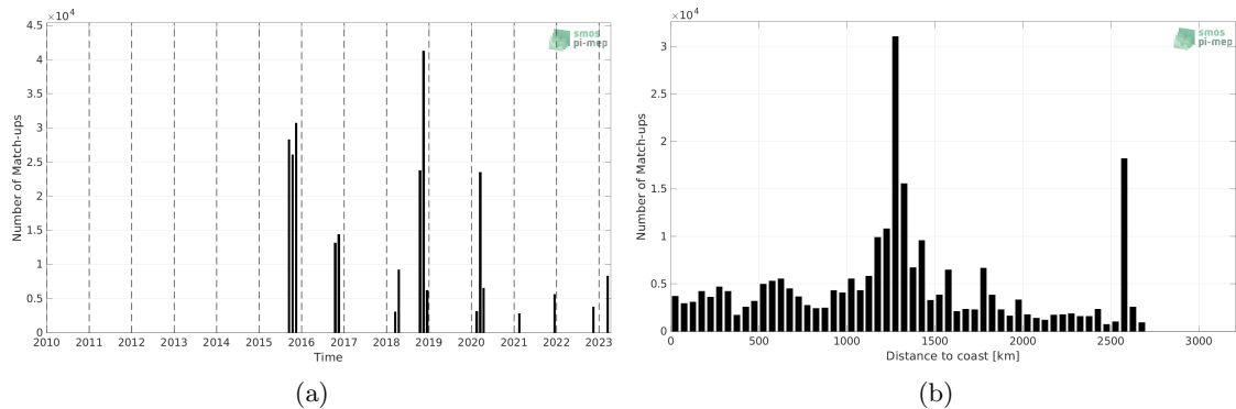
Figure 1: Number of match-ups between TSG (SAMOS) and SMAP SSS L2 v5.0 (JPL) SSS as a function of time (a) and as function of the distance to coast (b) over the South Atlantic Ocean Pi-MEP region and for the full satellite product period.
