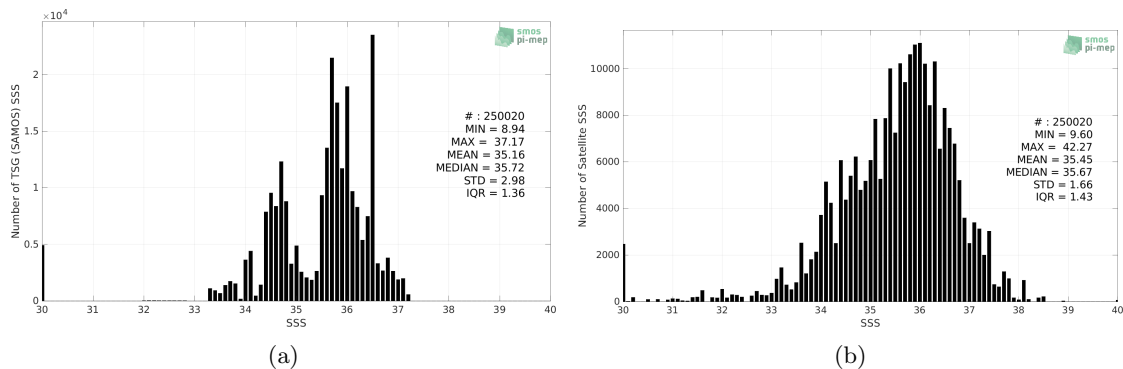
Figure 2: Histograms of SSS from TSG (SAMOS) (a) and SMAP SSS L2 v5.0 (JPL) (b) considering all match-up pairs per bins of 0.1 over the South Atlantic Ocean Pi-MEP region and for the full satellite product period.
