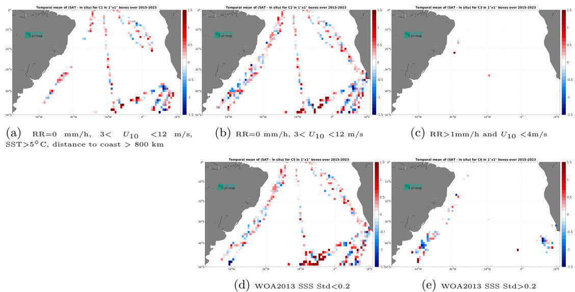
Figure 14: Temporal mean gridded over spatial boxes of size 1^\circ \times 1^\circ of \Delta SSS (SMAP SSS L2 v5.0 (JPL) - TSG (Polarstern)) for 5 different subdatasets corresponding to:RR=0 mm/h, 3 < U_{10} < 12 m/s, SST>5°C, distance to coast > 800 km (a), RR=0 mm/h, 3 < U_{10} < 12 m/s (b), RR>1mm/h and U_{10} < 4 m/s (c), WOA2013 SSS Std<0.2 (d), WOA2013 SSS Std>0.2 (e).
