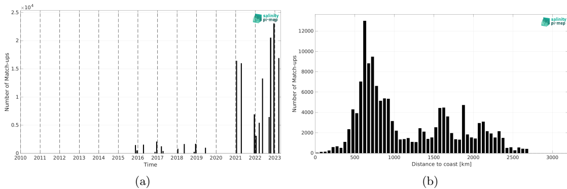
Figure 2: Number of match-ups between TSG (Polarstern) and SMAP SSS L2 v5.0 (JPL) SSS as a function of time (a) and as function of the distance to coast (b) over the South Atlantic Ocean Pi-MEP region and for the full satellite product period.
