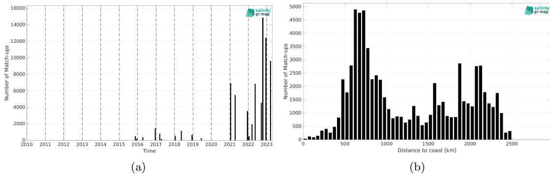
Figure 2: Number of match-ups between TSG (Polarstern) and SMAP SSS L2 v5.0 (JPL) SSS as a function of time (a) and as function of the distance to coast (b) over the South Atlantic Ocean Pi-MEP region and for the full satellite product period.
