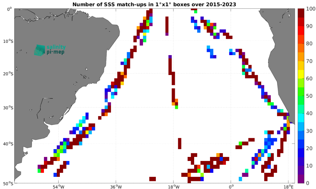
Figure 5: Number of SSS match-ups between TSG (Polarstern) SSS and the SMAP SSS L2 v5.0 (JPL) SSS product for the South Atlantic Ocean Pi-MEP region over 1^\circ \times 1^\circ boxes and for the full satellite product period.
