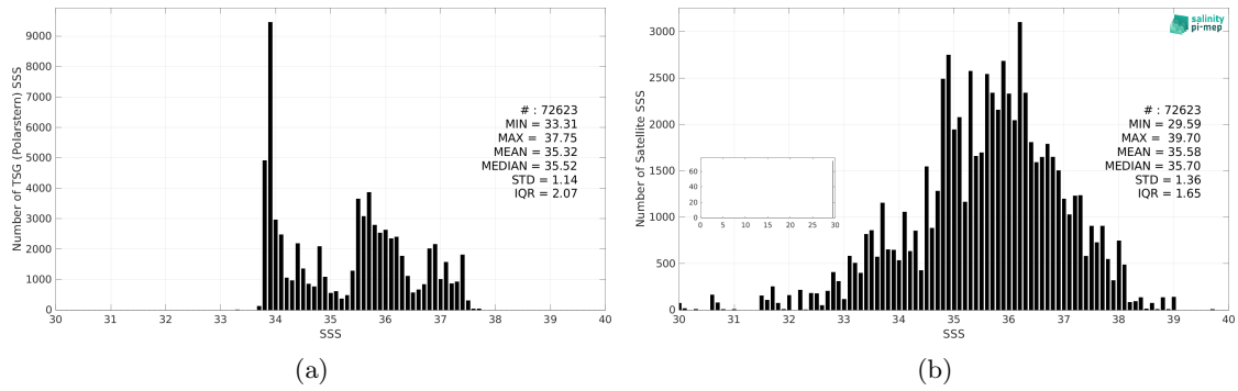
Figure 3: Histograms of SSS from TSG (Polarstern) (a) and SMAP SSS L2 v5.0 (JPL) (b) considering all match-up pairs per bins of 0.1 over the South Atlantic Ocean Pi-MEP region and for the full satellite product period.
