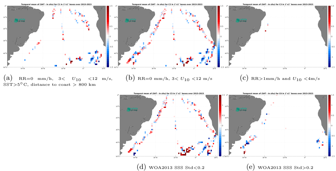
Figure 14: Temporal mean gridded over spatial boxes of size 1^\circ \times 1^\circ of \Delta\text{SSS} (SMAP SSS L2 v5.0 (JPL) - TSG (Polarstern)) for 5 different subdatasets corresponding to:RR=0 mm/h, 3 < U_{10} < 12 m/s, SST >5^\circ\text{C} , distance to coast > 800 km (a), RR=0 mm/h, 3 < U_{10} < 12 m/s (b), RR >1 mm/h and U_{10} < 4 m/s (c), WOA2013 SSS Std <0.2 (d), WOA2013 SSS Std >0.2 (e).
