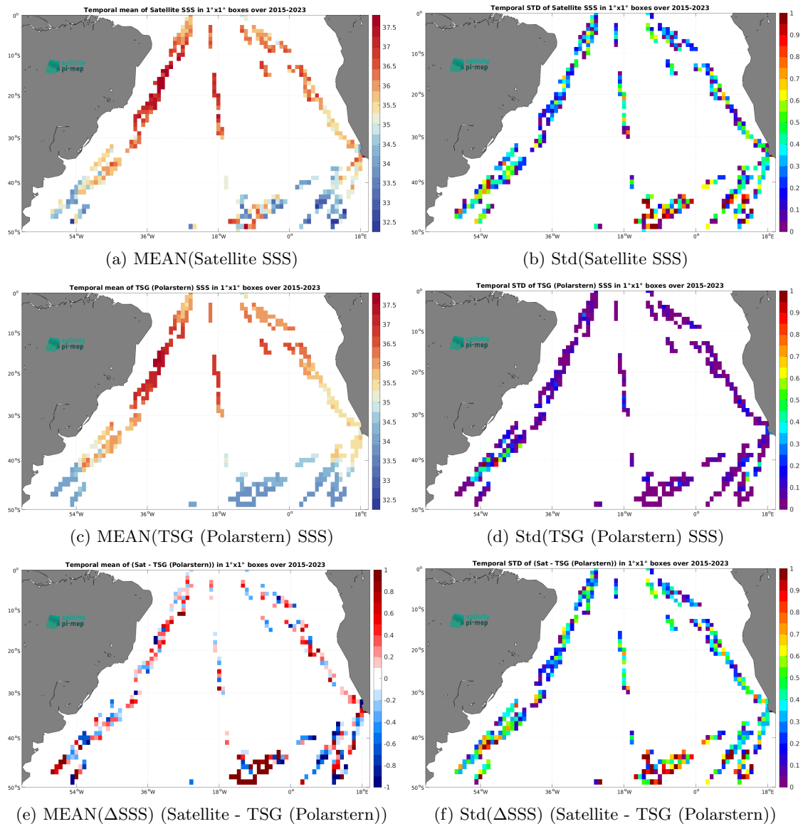
Figure 7: Temporal mean (left) and Std (right) of SSS from SMAP SSS L2 v5.0 (JPL) (top), TSG (Polarstern) (middle), and of \Delta SSS (Satellite - TSG (Polarstern)). Only match-up pairs are used to generate these maps.
