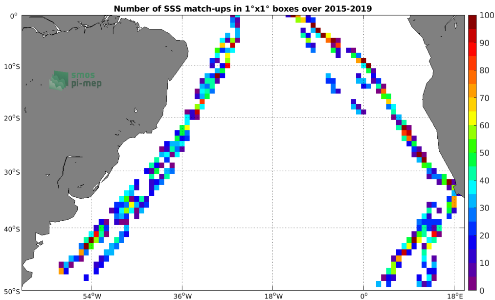
Figure 4: Number of SSS match-ups between TSG (Polarstern) SSS and the SMAP SSS L2 v5.0 (JPL) SSS product for the South Atlantic Ocean Pi-MEP region over 1°x1° boxes and for the full satellite product period.
