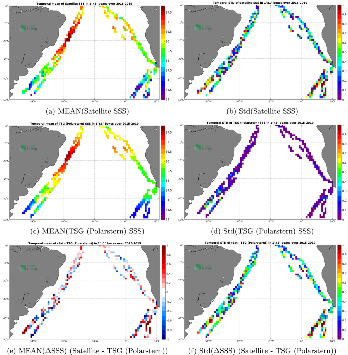
Figure 6: Temporal mean (left) and Std (right) of SSS from SMAP SSS L2 v5.0 (JPL) (top), TSG (Polarstern) (middle), and of \Delta SSS (Satellite - TSG (Polarstern)). Only match-up pairs are used to generate these maps.
