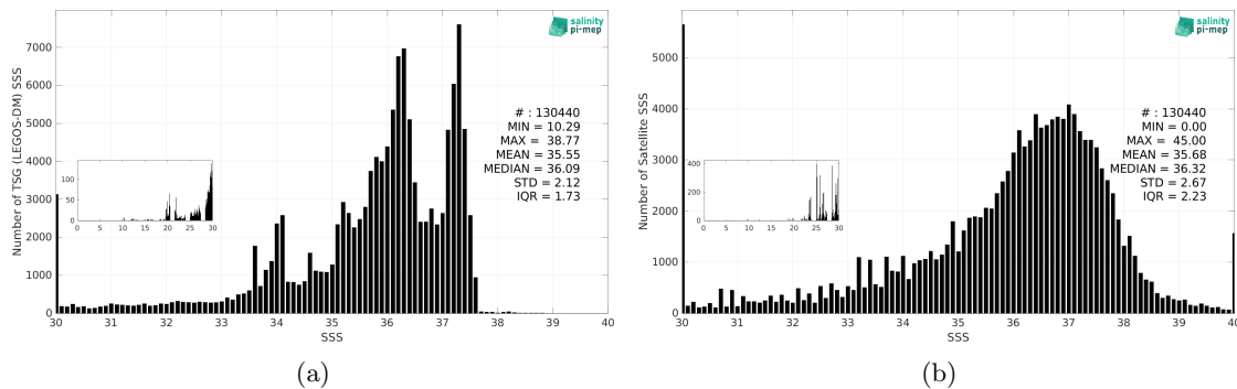
Figure 3: Histograms of SSS from TSG (LEGOS-DM) (a) and SMAP SSS L2 v5.0 (JPL) (b) considering all match-up pairs per bins of 0.1 over the South Atlantic Ocean Pi-MEP region and for the full satellite product period.
