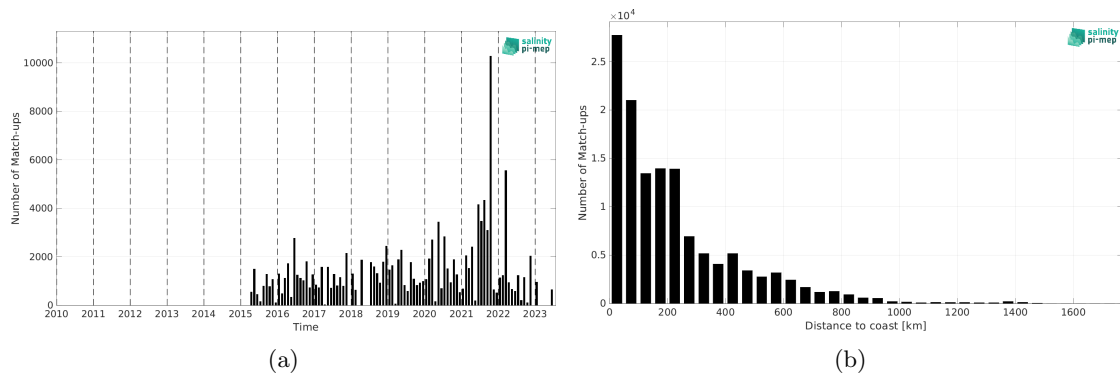
Figure 2: Number of match-ups between TSG (LEGOS-DM) and SMAP SSS L2 v5.0 (JPL) SSS as a function of time (a) and as function of the distance to coast (b) over the South Atlantic Ocean Pi-MEP region and for the full satellite product period.
