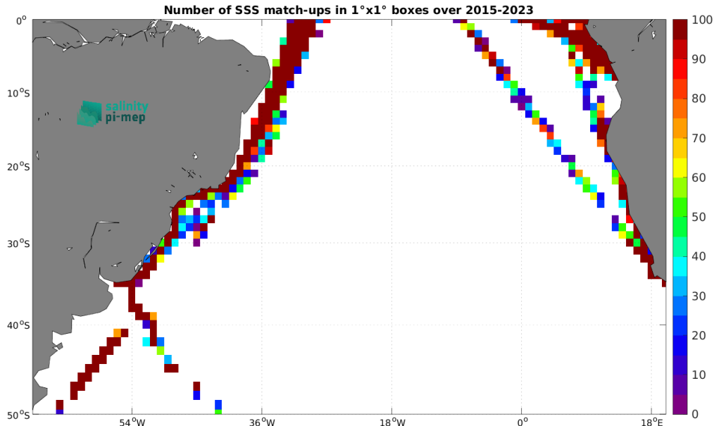
Figure 5: Number of SSS match-ups between TSG (LEGOS-DM) SSS and the SMAP SSS L2 v5.0 (JPL) SSS product for the South Atlantic Ocean Pi-MEP region over 1^\circ \times 1^\circ boxes and for the full satellite product period.
