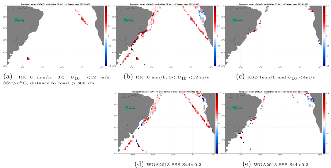
Figure 14: Temporal mean gridded over spatial boxes of size 1^\circ \times 1^\circ of \Delta SSS (SMAP SSS L2 v5.0 (JPL) - TSG (LEGOS-DM)) for 5 different subdatasets corresponding to:RR=0 mm/h, 3 < U_{10} < 12 m/s, SST>5°C, distance to coast > 800 km (a), RR=0 mm/h, 3 < U_{10} < 12 m/s (b), RR>1mm/h and U_{10} < 4 m/s (c), WOA2013 SSS Std<0.2 (d), WOA2013 SSS Std>0.2 (e).
