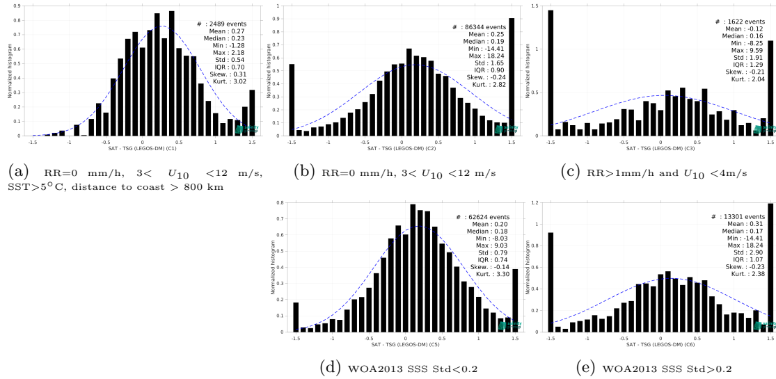
Figure 13: Normalized histogram of \Delta\text{SSS} (SMAP SSS L2 v5.0 (JPL) - TSG (LEGOS-DM)) for 5 different subdatasets corresponding to: RR=0 mm/h, 3 < U_{10} < 12 m/s, SST>5°C, distance to coast > 800 km (a), RR=0 mm/h, 3 < U_{10} < 12 m/s (b), RR>1mm/h and U_{10} < 4 m/s (c), WOA2013 SSS Std<0.2 (d), WOA2013 SSS Std>0.2 (e).
