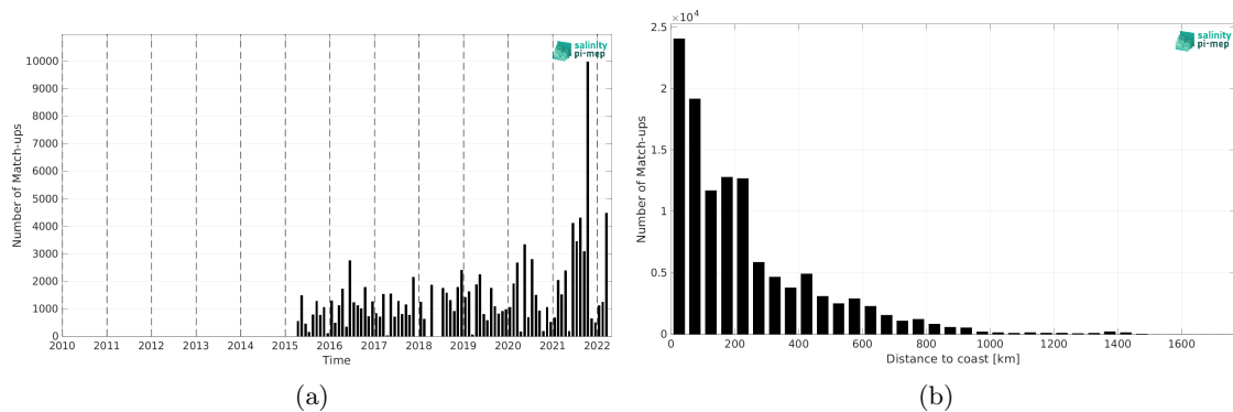
Figure 1: Number of match-ups between TSG (LEGOS-DM) and SMAP SSS L2 v5.0 (JPL) SSS as a function of time (a) and as function of the distance to coast (b) over the South Atlantic Ocean Pi-MEP region and for the full satellite product period.
