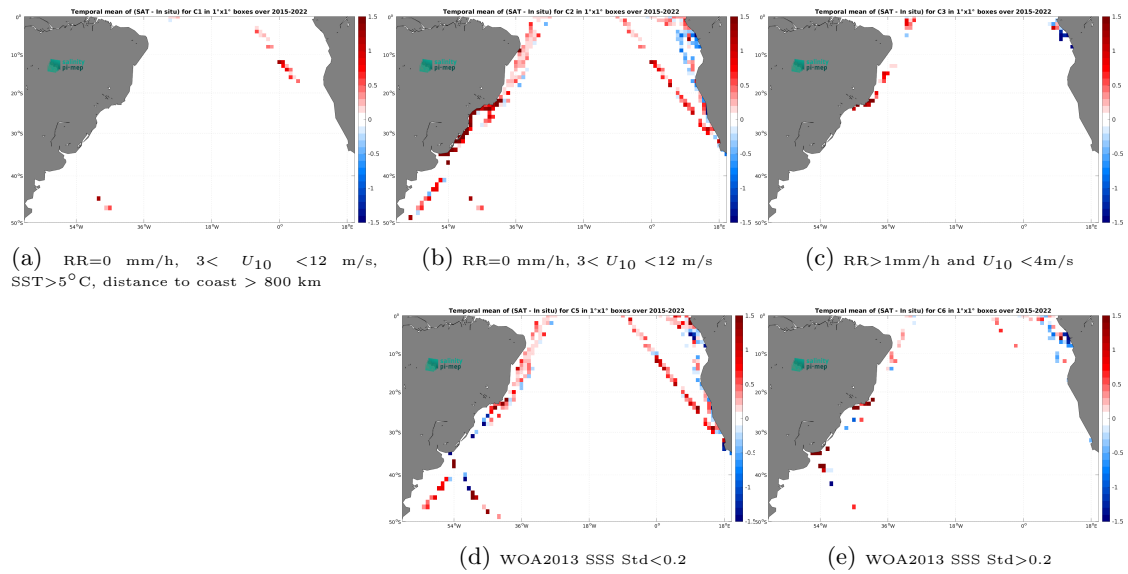
Figure 12: Temporal mean gridded over spatial boxes of size 1^\circ \times 1^\circ of \Delta\text{SSS} (SMAP SSS L2 v5.0 (JPL) - TSG (LEGOS-DM)) for 5 different subdatasets corresponding to:RR=0 mm/h, 3 < U_{10} < 12 m/s, \text{SST} > 5^\circ\text{C} , distance to coast > 800 km (a), RR=0 mm/h, 3 < U_{10} < 12 m/s (b), RR>1mm/h and U_{10} < 4\text{m/s} (c), WOA2013 SSS Std<0.2 (d), WOA2013 SSS Std>0.2 (e).
