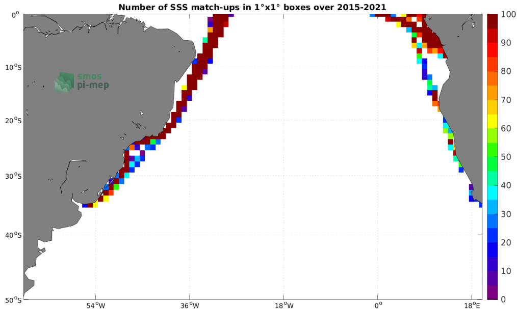
Figure 4: Number of SSS match-ups between TSG (LEGOS-DM) SSS and the SMAP SSS L2 v5.0 (JPL) SSS product for the South Atlantic Ocean Pi-MEP region over 1^\circ \times 1^\circ boxes and for the full satellite product period.
