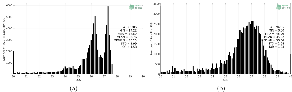
Figure 2: Histograms of SSS from TSG (LEGOS-DM) (a) and SMAP SSS L2 v5.0 (JPL) (b) considering all match-up pairs per bins of 0.1 over the South Atlantic Ocean Pi-MEP region and for the full satellite product period.
