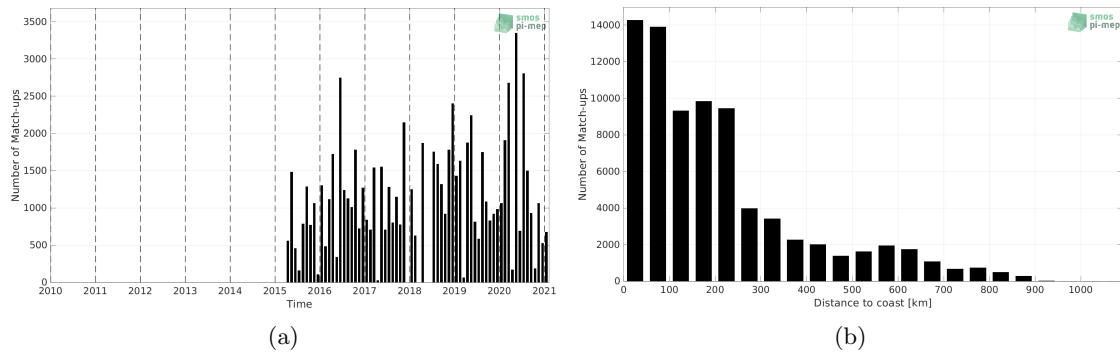
Figure 1: Number of match-ups between TSG (LEGOS-DM) and SMAP SSS L2 v5.0 (JPL) SSS as a function of time (a) and as function of the distance to coast (b) over the South Atlantic Ocean Pi-MEP region and for the full satellite product period.
