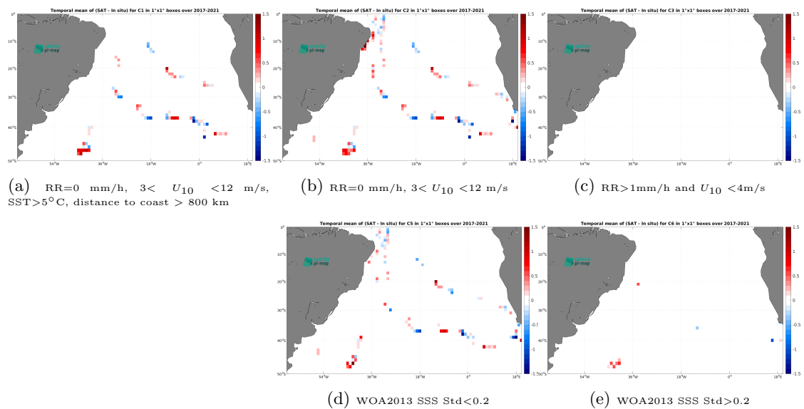
Figure 14: Temporal mean gridded over spatial boxes of size 1^\circ \times 1^\circ of \Delta\text{SSS} (SMAP SSS L2 v5.0 (JPL) - TSG (GOSUD-Sailing-ship)) for 5 different subdatasets corresponding to:RR=0 mm/h, 3 < U_{10} < 12 m/s, SST>5°C, distance to coast > 800 km (a), RR=0 mm/h, 3 < U_{10} < 12 m/s (b), RR>1mm/h and U_{10} < 4 m/s (c), WOA2013 SSS Std<0.2 (d), WOA2013 SSS Std>0.2 (e).
