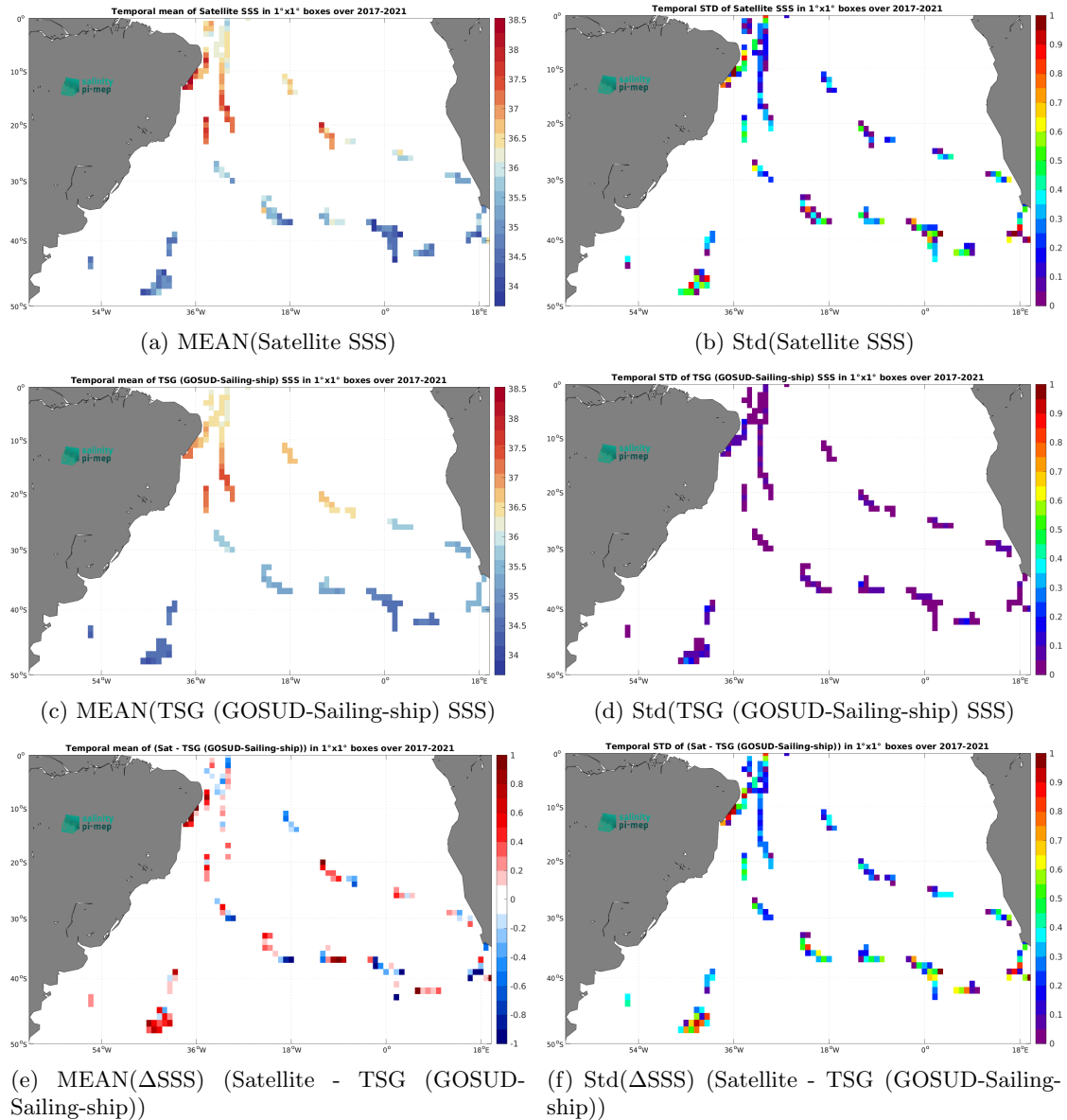
Figure 7: Temporal mean (left) and Std (right) of SSS from SMAP SSS L2 v5.0 (JPL) (top), TSG (GOSUD-Sailing-ship) (middle), and of \Delta SSS (Satellite - TSG (GOSUD-Sailing-ship)). Only match-up pairs are used to generate these maps.
