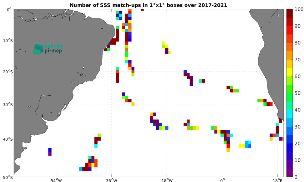
Figure 5: Number of SSS match-ups between TSG (GOSUD-Sailing-ship) SSS and the SMAP SSS L2 v5.0 (JPL) SSS product for the South Atlantic Ocean Pi-MEP region over 1^\circ \times 1^\circ boxes and for the full satellite product period.
