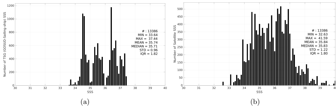
Figure 3: Histograms of SSS from TSG (GOSUD-Sailing-ship) (a) and SMAP SSS L2 v5.0 (JPL) (b) considering all match-up pairs per bins of 0.1 over the South Atlantic Ocean Pi-MEP region and for the full satellite product period.
