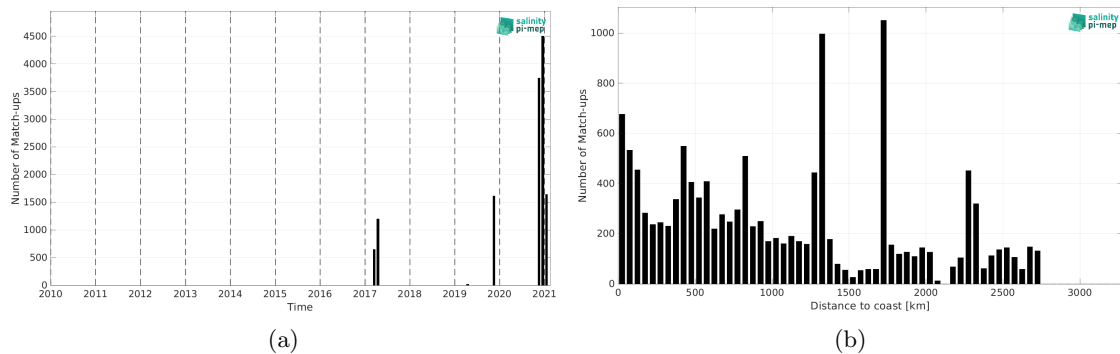
Figure 2: Number of match-ups between TSG (GOSUD-Sailing-ship) and SMAP SSS L2 v5.0 (JPL) SSS as a function of time (a) and as function of the distance to coast (b) over the South Atlantic Ocean Pi-MEP region and for the full satellite product period.
