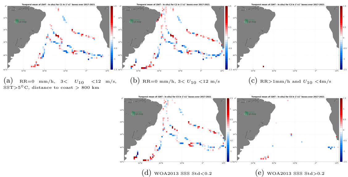
Figure 12: Temporal mean gridded over spatial boxes of size 1^\circ \times 1^\circ of \Delta\text{SSS} (SMAP SSS L2 v5.0 (JPL) - TSG (GOSUD-Sailing-ship)) for 5 different subdatasets corresponding to:RR=0 mm/h, 3 < U_{10} < 12 m/s, SST >5^\circ\text{C} , distance to coast > 800 km (a), RR=0 mm/h, 3 < U_{10} < 12 m/s (b), RR >1 mm/h and U_{10} < 4 m/s (c), WOA2013 SSS Std <0.2 (d), WOA2013 SSS Std >0.2 (e).
