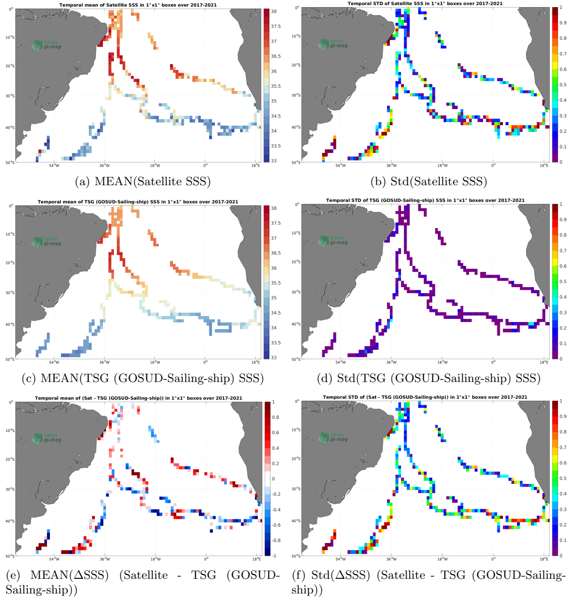
Figure 6: Temporal mean (left) and Std (right) of SSS from SMAP SSS L2 v5.0 (JPL) (top), TSG (GOSUD-Sailing-ship) (middle), and of \Delta SSS (Satellite - TSG (GOSUD-Sailing-ship)). Only match-up pairs are used to generate these maps.
