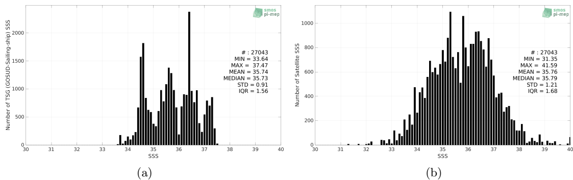
Figure 2: Histograms of SSS from TSG (GOSUD-Sailing-ship) (a) and SMAP SSS L2 v5.0 (JPL) (b) considering all match-up pairs per bins of 0.1 over the South Atlantic Ocean Pi-MEP region and for the full satellite product period.
