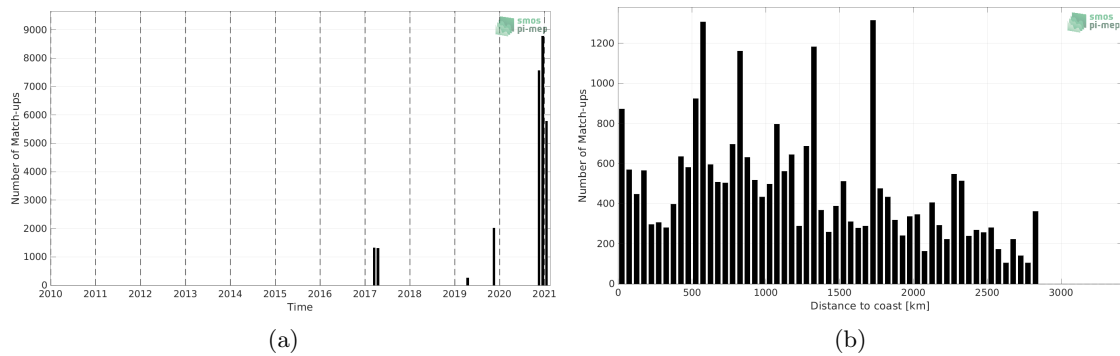
Figure 1: Number of match-ups between TSG (GOSUD-Sailing-ship) and SMAP SSS L2 v5.0 (JPL) SSS as a function of time (a) and as function of the distance to coast (b) over the South Atlantic Ocean Pi-MEP region and for the full satellite product period.
