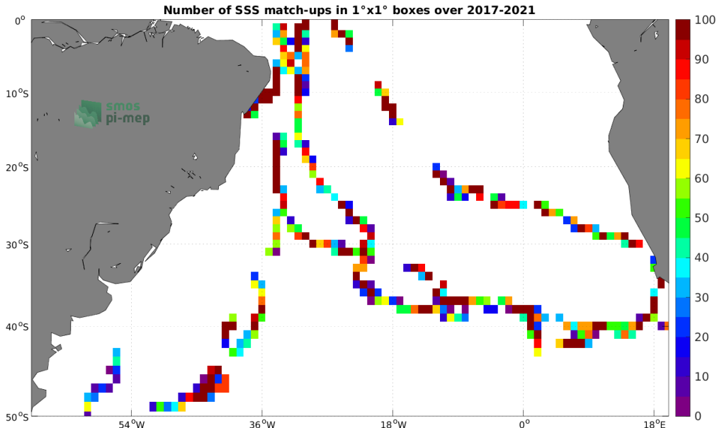
Figure 4: Number of SSS match-ups between TSG (GOSUD-Sailing-ship) SSS and the SMAP SSS L2 v5.0 (JPL) SSS product for the South Atlantic Ocean Pi-MEP region over 1^\circ \times 1^\circ boxes and for the full satellite product period.
