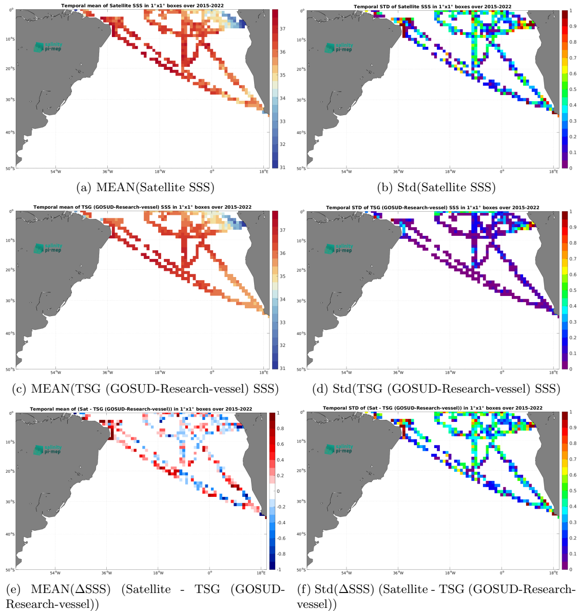
Figure 7: Temporal mean (left) and Std (right) of SSS from SMAP SSS L2 v5.0 (JPL) (top), TSG (GOSUD-Research-vessel) (middle), and of \Delta SSS (Satellite - TSG (GOSUD-Research-vessel)). Only match-up pairs are used to generate these maps.
