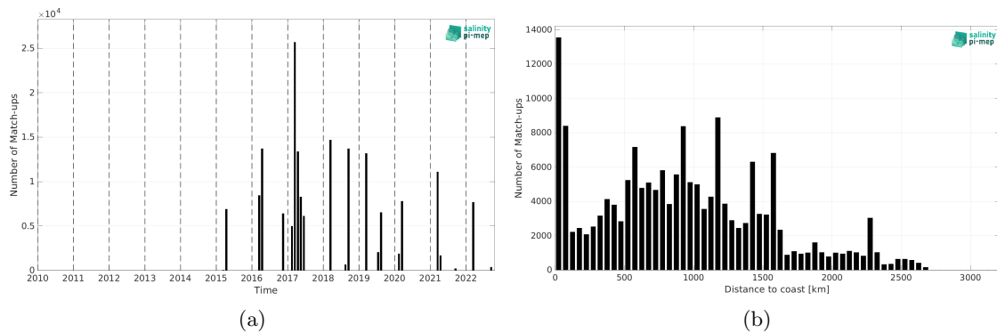
Figure 2: Number of match-ups between TSG (GOSUD-Research-vessel) and SMAP SSS L2 v5.0 (JPL) SSS as a function of time (a) and as function of the distance to coast (b) over the South Atlantic Ocean Pi-MEP region and for the full satellite product period.
