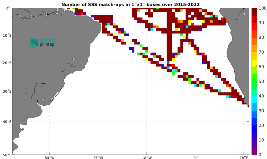
Figure 5: Number of SSS match-ups between TSG (GOSUD-Research-vessel) SSS and the SMAP SSS L2 v5.0 (JPL) SSS product for the South Atlantic Ocean Pi-MEP region over 1^\circ \times 1^\circ boxes and for the full satellite product period.
