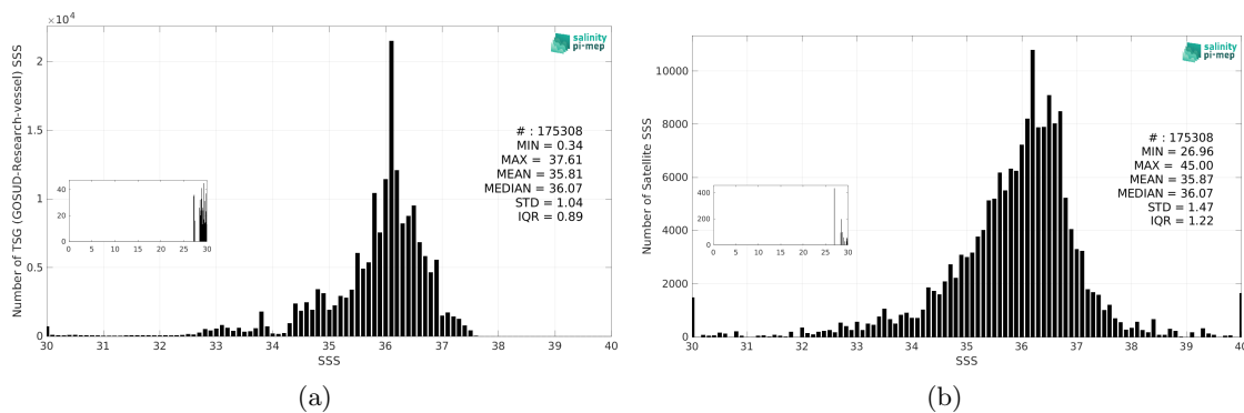
Figure 3: Histograms of SSS from TSG (GOSUD-Research-vessel) (a) and SMAP SSS L2 v5.0 (JPL) (b) considering all match-up pairs per bins of 0.1 over the South Atlantic Ocean Pi-MEP region and for the full satellite product period.
