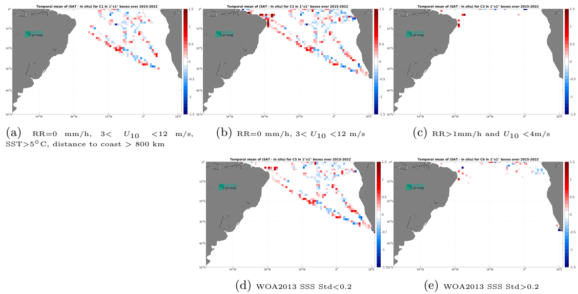
Figure 14: Temporal mean gridded over spatial boxes of size 1^\circ \times 1^\circ of \Delta SSS (SMAP SSS L2 v5.0 (JPL) - TSG (GOSUD-Research-vessel)) for 5 different subdatasets corresponding to:RR=0 mm/h, 3 < U_{10} < 12 m/s, SST>5°C, distance to coast > 800 km (a), RR=0 mm/h, 3 < U_{10} < 12 m/s (b), RR>1mm/h and U_{10} < 4 m/s (c), WOA2013 SSS Std<0.2 (d), WOA2013 SSS Std>0.2 (e).
