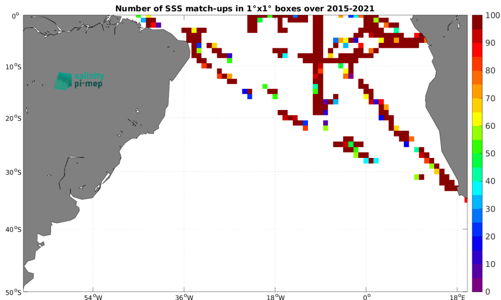
Figure 5: Number of SSS match-ups between TSG (GOSUD-Research-vessel) SSS and the SMAP SSS L2 v5.0 (JPL) SSS product for the South Atlantic Ocean Pi-MEP region over 1^{\circ} \times 1^{\circ} boxes and for the full satellite product period.
