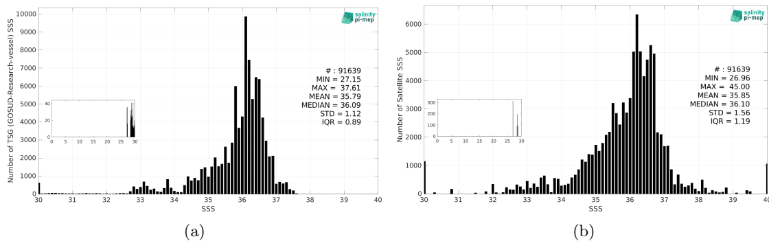
Figure 3: Histograms of SSS from TSG (GOSUD-Research-vessel) (a) and SMAP SSS L2 v5.0 (JPL) (b) considering all match-up pairs per bins of 0.1 over the South Atlantic Ocean Pi-MEP region and for the full satellite product period.
