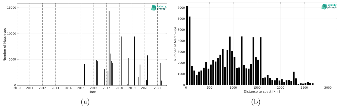
Figure 2: Number of match-ups between TSG (GOSUD-Research-vessel) and SMAP SSS L2 v5.0 (JPL) SSS as a function of time (a) and as function of the distance to coast (b) over the South Atlantic Ocean Pi-MEP region and for the full satellite product period.
