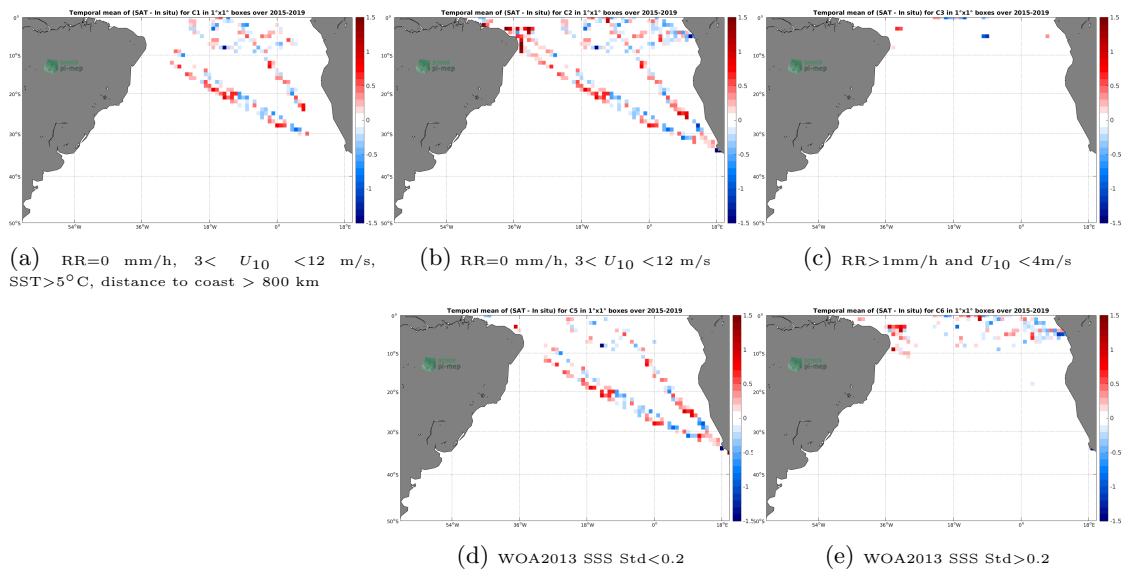
Figure 12: Temporal mean gridded over spatial boxes of size 1°x1° of \Delta SSS (SMAP SSS L2 v5.0 (JPL) - TSG (GOSUD-Research-vessel)) for 5 different subdatasets corresponding to:RR=0 mm/h, 3 < U_{10} < 12 m/s, SST>5°C, distance to coast > 800 km (a), RR=0 mm/h, 3 < U_{10} < 12 m/s (b), RR>1mm/h and U_{10} < 4 m/s (c), WOA2013 SSS Std<0.2 (d), WOA2013 SSS Std>0.2 (e).
