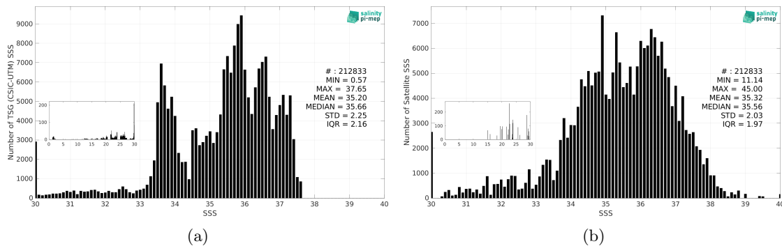
Figure 3: Histograms of SSS from TSG (CSIC-UTM) (a) and SMAP SSS L2 v5.0 (JPL) (b) considering all match-up pairs per bins of 0.1 over the South Atlantic Ocean Pi-MEP region and for the full satellite product period.
