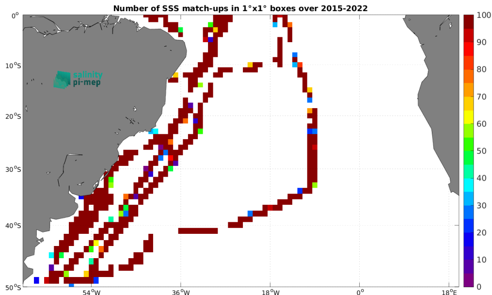
Figure 5: Number of SSS match-ups between TSG (CSIC-UTM) SSS and the SMAP SSS L2 v5.0 (JPL) SSS product for the South Atlantic Ocean Pi-MEP region over 1^\circ \times 1^\circ boxes and for the full satellite product period.
