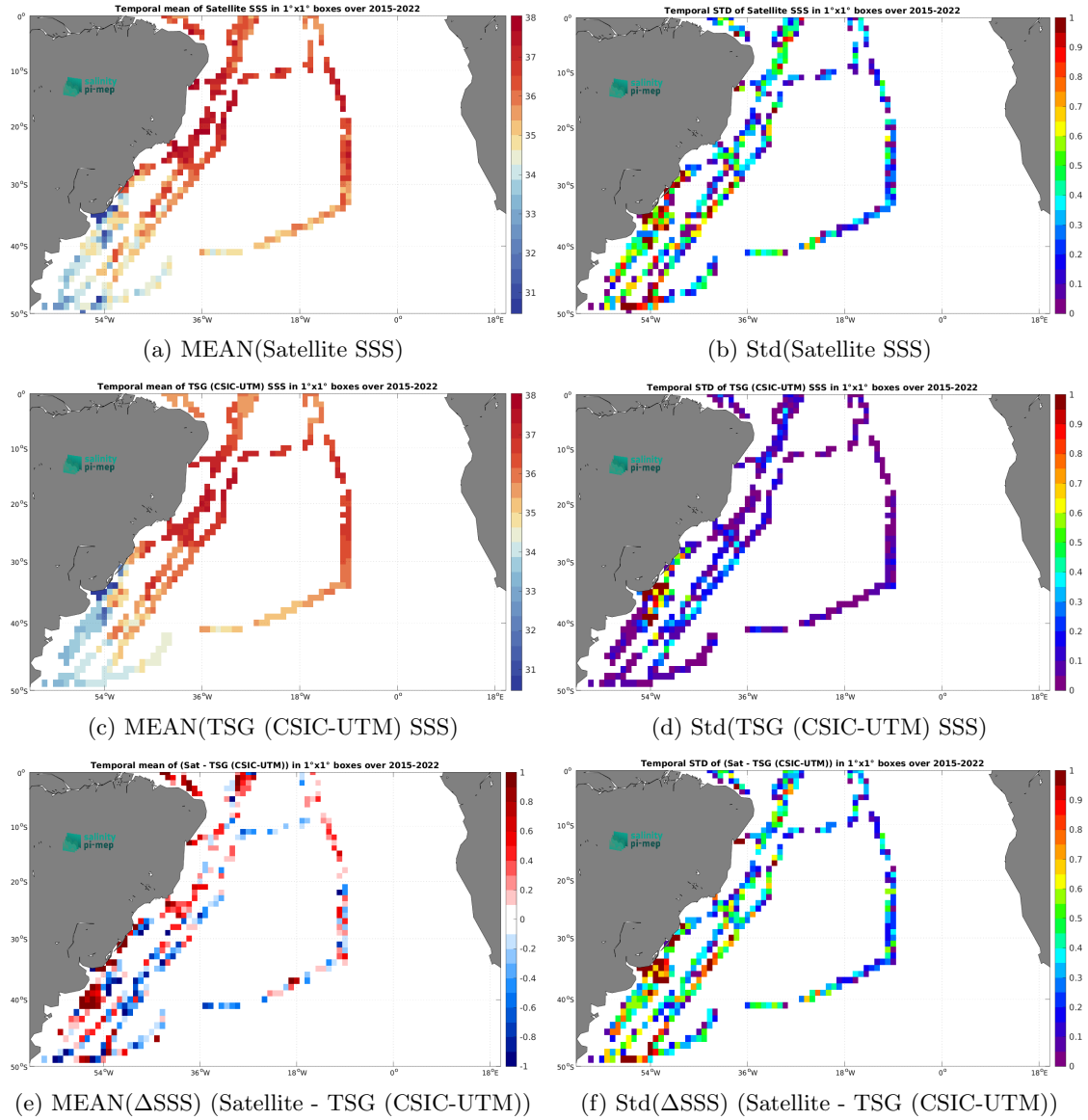
Figure 7: Temporal mean (left) and Std (right) of SSS from SMAP SSS L2 v5.0 (JPL) (top), TSG (CSIC-UTM) (middle), and of \Delta SSS (Satellite - TSG (CSIC-UTM)). Only match-up pairs are used to generate these maps.
