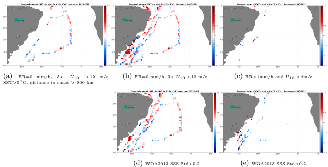
Figure 14: Temporal mean gridded over spatial boxes of size 1^\circ \times 1^\circ of \Delta SSS (SMAP SSS L2 v5.0 (JPL) - TSG (CSIC-UTM)) for 5 different subdatasets corresponding to:RR=0 mm/h, 3 < U_{10} < 12 m/s, SST>5°C, distance to coast > 800 km (a), RR=0 mm/h, 3 < U_{10} < 12 m/s (b), RR>1mm/h and U_{10} < 4 m/s (c), WOA2013 SSS Std<0.2 (d), WOA2013 SSS Std>0.2 (e).
