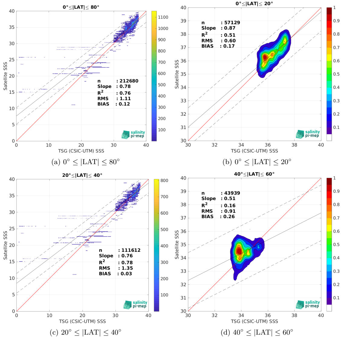
Figure 10: Contour maps of the concentration of SMAP SSS L2 v5.0 (JPL) SSS (y-axis) versus TSG (CSIC-UTM) SSS (x-axis) at match-up pairs for different latitude bands. For each plot, the red line shows x=y . The black thin and dashed lines indicate a linear fit through the data cloud and the \pm 95\% confidence levels, respectively. The number match-up pairs n , the slope and R^2 coefficient of the linear fit, the root mean square (RMS) and the mean bias between satellite and in situ data are indicated for each latitude band in each plots.
