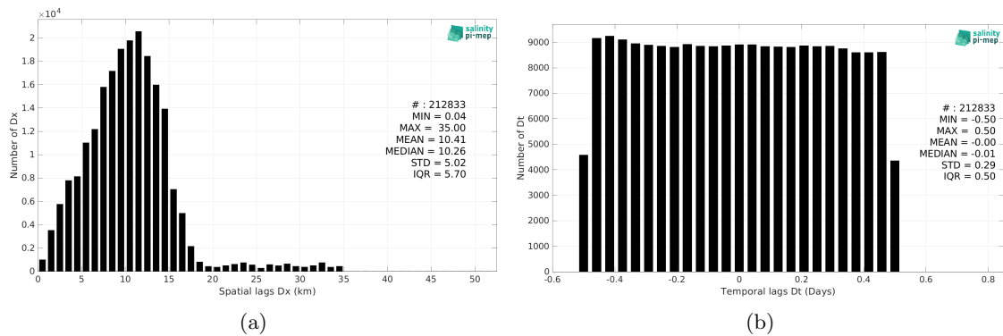
Figure 6: Histograms of the spatial (a) and temporal (b) lags between the location/time of the TSG (CSIC-UTM) measurement and the date of the corresponding SMAP SSS L2 v5.0 (JPL) SSS pixel.
