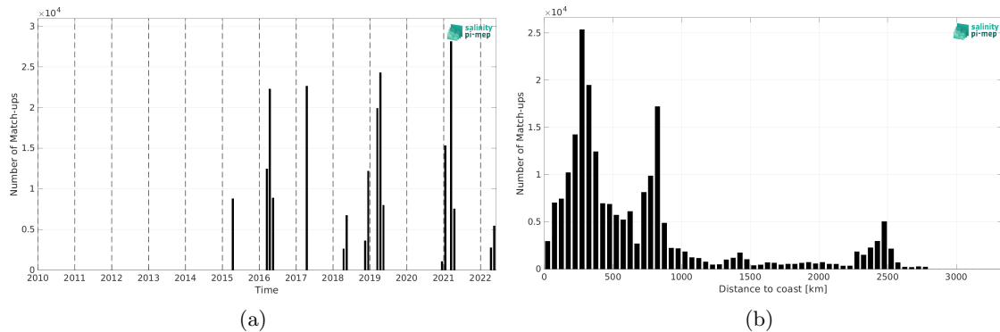
Figure 2: Number of match-ups between TSG (CSIC-UTM) and SMAP SSS L2 v5.0 (JPL) SSS as a function of time (a) and as function of the distance to coast (b) over the South Atlantic Ocean Pi-MEP region and for the full satellite product period.
