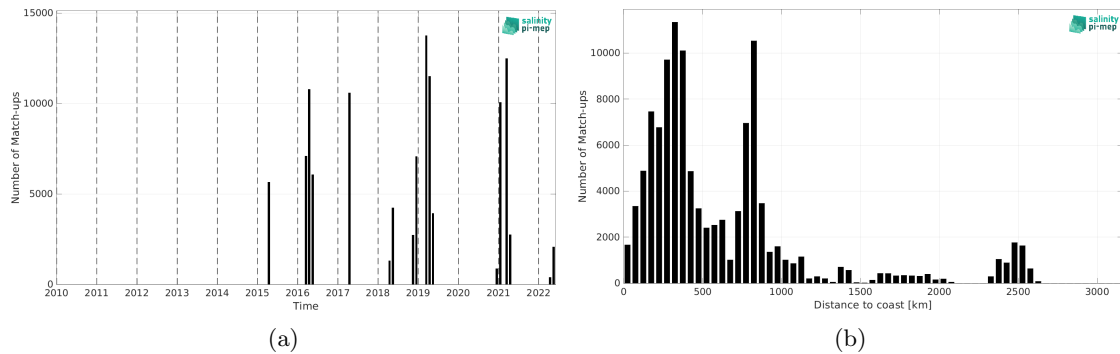
Figure 2: Number of match-ups between TSG (CSIC-UTM) and SMAP SSS L2 v5.0 (JPL) SSS as a function of time (a) and as function of the distance to coast (b) over the South Atlantic Ocean Pi-MEP region and for the full satellite product period.
