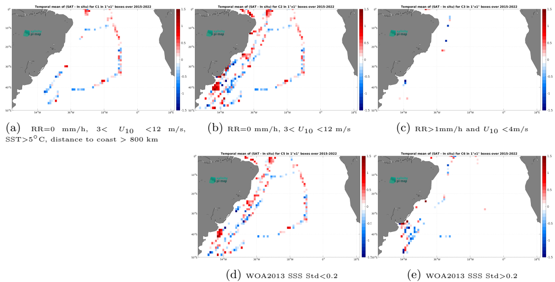
Figure 12: Temporal mean gridded over spatial boxes of size 1^\circ \times 1^\circ of \Delta SSS (SMAP SSS L2 v5.0 (JPL) - TSG (CSIC-UTM)) for 5 different subdatasets corresponding to:RR=0 mm/h, 3 < U_{10} < 12 m/s, SST >5^\circ\text{C} , distance to coast > 800 km (a), RR=0 mm/h, 3 < U_{10} < 12 m/s (b), RR >1 mm/h and U_{10} < 4 m/s (c), WOA2013 SSS Std <0.2 (d), WOA2013 SSS Std >0.2 (e).
