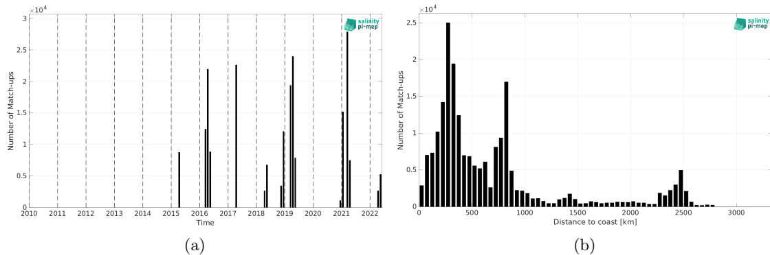
Figure 1: Number of match-ups between TSG (CSIC-UTM) and SMAP SSS L2 v5.0 (JPL) SSS as a function of time (a) and as function of the distance to coast (b) over the South Atlantic Ocean Pi-MEP region and for the full satellite product period.
