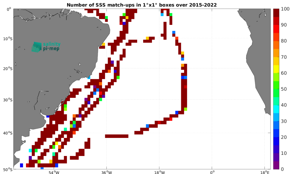
Figure 4: Number of SSS match-ups between TSG (CSIC-UTM) SSS and the SMAP SSS L2 v5.0 (JPL) SSS product for the South Atlantic Ocean Pi-MEP region over 1^\circ \times 1^\circ boxes and for the full satellite product period.
