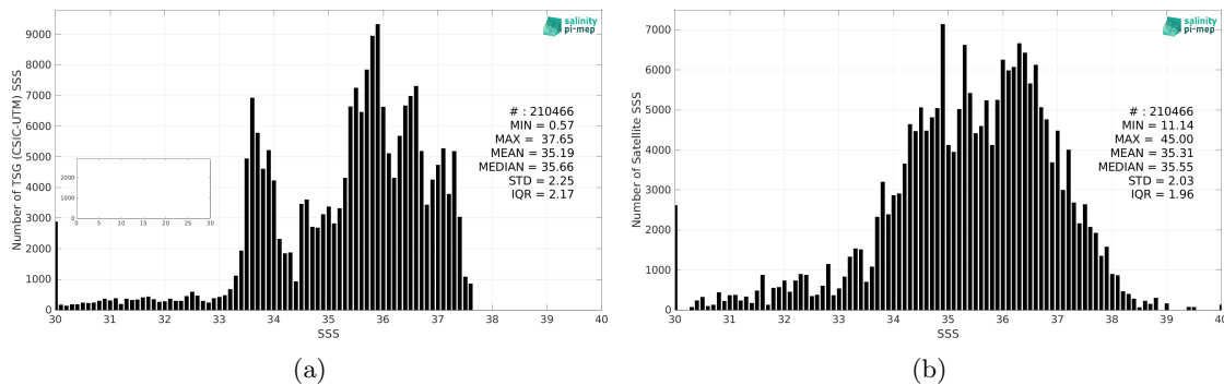
Figure 2: Histograms of SSS from TSG (CSIC-UTM) (a) and SMAP SSS L2 v5.0 (JPL) (b) considering all match-up pairs per bins of 0.1 over the South Atlantic Ocean Pi-MEP region and for the full satellite product period.
