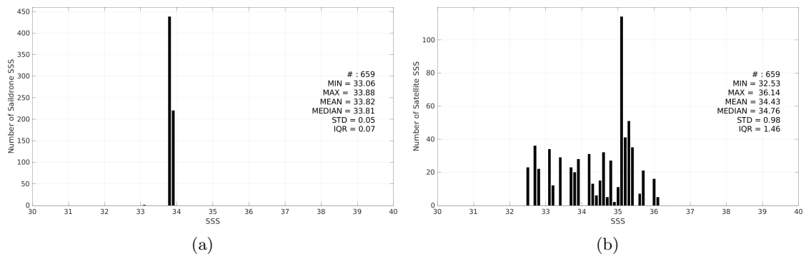
Figure 3: Histograms of SSS from Saildrone (a) and SMAP SSS L2 v5.0 (JPL) (b) considering all match-up pairs per bins of 0.1 over the South Atlantic Ocean Pi-MEP region and for the full satellite product period.
