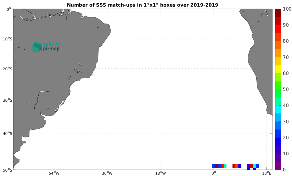
Figure 5: Number of SSS match-ups between Saildrone SSS and the SMAP SSS L2 v5.0 (JPL) SSS product for the South Atlantic Ocean Pi-MEP region over 1^{\circ} \times 1^{\circ} boxes and for the full satellite product period.
