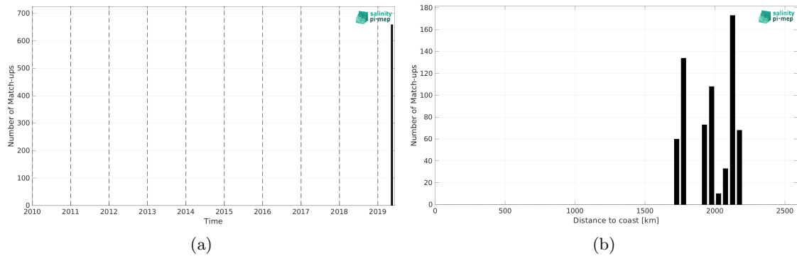
Figure 2: Number of match-ups between Saildrone and SMAP SSS L2 v5.0 (JPL) SSS as a function of time (a) and as function of the distance to coast (b) over the South Atlantic Ocean Pi-MEP region and for the full satellite product period.
