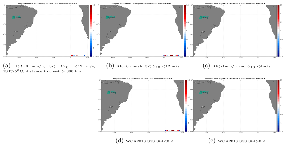
Figure 14: Temporal mean gridded over spatial boxes of size 1^\circ \times 1^\circ of \Delta SSS (SMAP SSS L2 v5.0 (JPL) - Saldrone) for 5 different subdatasets corresponding to:RR=0 mm/h, 3 < U_{10} < 12 m/s, SST >5^\circ\text{C} , distance to coast > 800 km (a), RR=0 mm/h, 3 < U_{10} < 12 m/s (b), RR >1 mm/h and U_{10} < 4 m/s (c), WOA2013 SSS Std <0.2 (d), WOA2013 SSS Std >0.2 (e).
