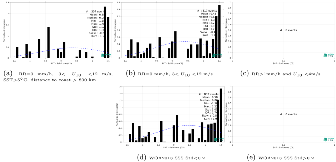
Figure 13: Normalized histogram of \Delta SSS (SMAP SSS L2 v5.0 (JPL) - Sairdrone) for 5 different subdatasets corresponding to: RR=0 mm/h, 3 < U_{10} < 12 m/s, SST > 5°C, distance to coast > 800 km (a), RR=0 mm/h, 3 < U_{10} < 12 m/s (b), RR > 1mm/h and U_{10} < 4 m/s (c), WOA2013 SSS Std < 0.2 (d), WOA2013 SSS Std > 0.2 (e).
