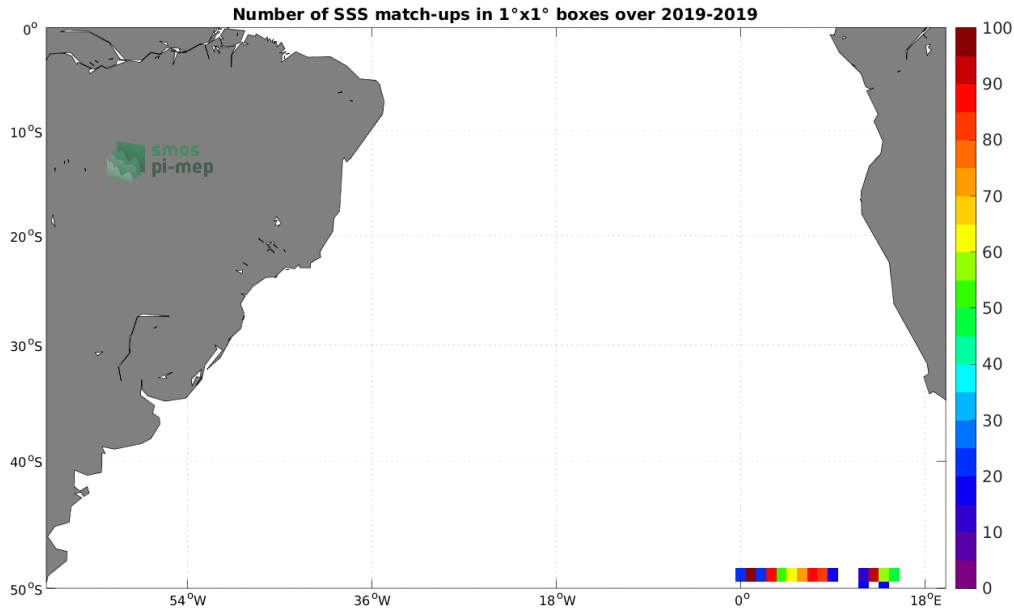
Figure 4: Number of SSS match-ups between Saildrone SSS and the SMAP SSS L2 v5.0 (JPL) SSS product for the South Atlantic Ocean Pi-MEP region over 1°x1° boxes and for the full satellite product period.
