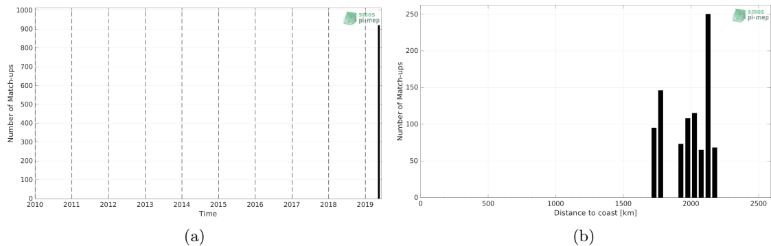
Figure 1: Number of match-ups between Saildrone and SMAP SSS L2 v5.0 (JPL) SSS as a function of time (a) and as function of the distance to coast (b) over the South Atlantic Ocean Pi-MEP region and for the full satellite product period.
