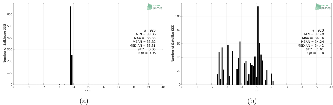
Figure 2: Histograms of SSS from Saildrone (a) and SMAP SSS L2 v5.0 (JPL) (b) considering all match-up pairs per bins of 0.1 over the South Atlantic Ocean Pi-MEP region and for the full satellite product period.
