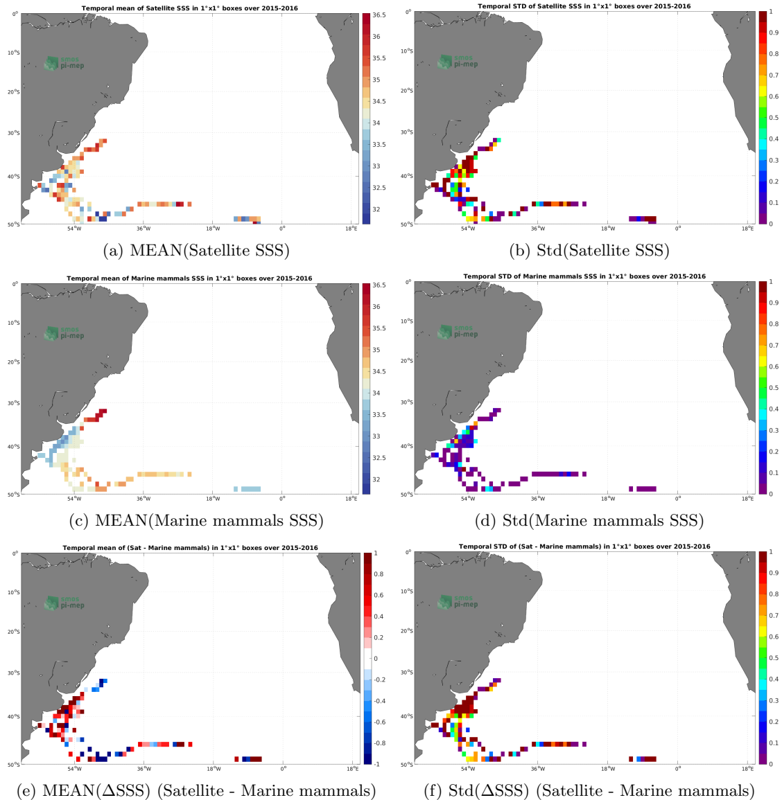
Figure 6: Temporal mean (left) and Std (right) of SSS from SMAP SSS L2 v5.0 (JPL) (top), Marine mammals (middle), and of \Delta SSS (Satellite - Marine mammals). Only match-up pairs are used to generate these maps.
