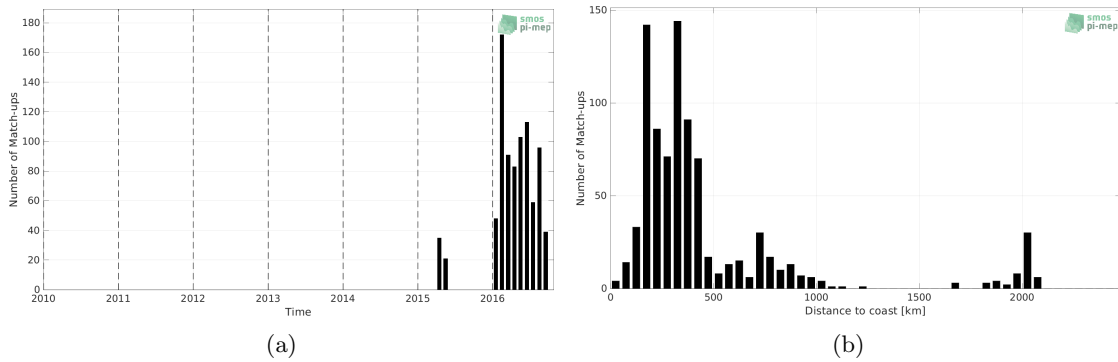
Figure 1: Number of match-ups between Marine mammals and SMAP SSS L2 v5.0 (JPL) SSS as a function of time (a) and as function of the distance to coast (b) over the South Atlantic Ocean Pi-MEP region and for the full satellite product period.
