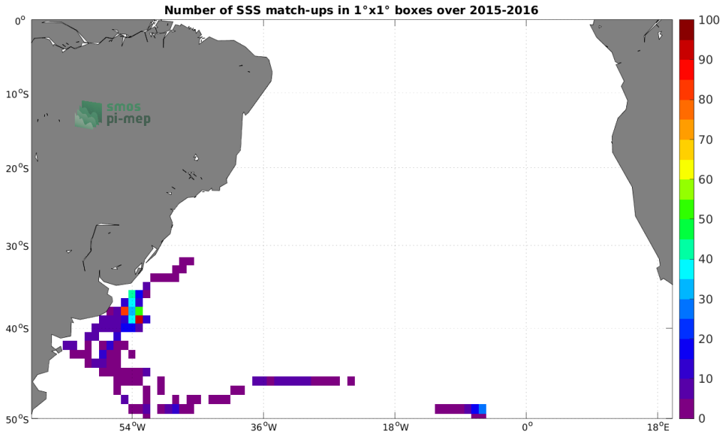
Figure 4: Number of SSS match-ups between Marine mammals SSS and the SMAP SSS L2 v5.0 (JPL) SSS product for the South Atlantic Ocean Pi-MEP region over 1^{\circ} \times 1^{\circ} boxes and for the full satellite product period.
