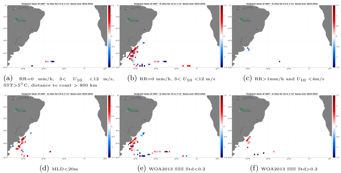
Figure 12: Temporal mean gridded over spatial boxes of size 1^\circ \times 1^\circ of \Delta SSS (SMAP SSS L2 v5.0 (JPL) - Marine mammals) for 6 different subdatasets corresponding to:RR=0 mm/h, 3 < U_{10} < 12 m/s, SST > 5^\circ\text{C} , distance to coast > 800 km (a), RR=0 mm/h, 3 < U_{10} < 12 m/s (b), RR > 1 mm/h and U_{10} < 4 m/s (c),MLD < 20 m (d),WOA2013 SSS Std < 0.2 (e),WOA2013 SSS Std > 0.2 (f).
