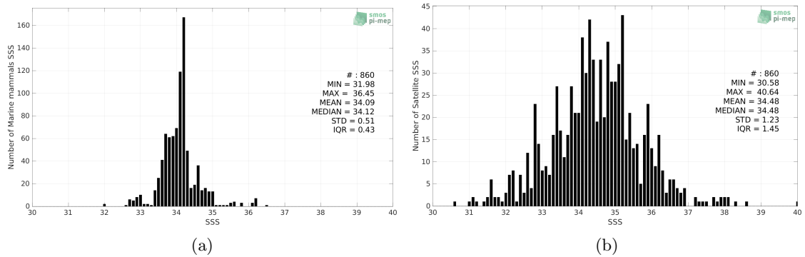
Figure 2: Histograms of SSS from Marine mammals (a) and SMAP SSS L2 v5.0 (JPL) (b) considering all match-up pairs per bins of 0.1 over the South Atlantic Ocean Pi-MEP region and for the full satellite product period.
