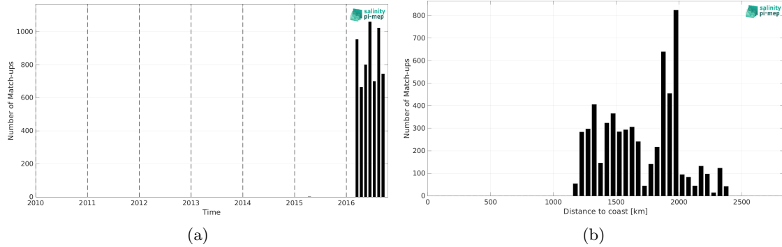
Figure 2: Number of match-ups between Surface drifters and SMAP SSS L2 v5.0 (JPL) SSS as a function of time (a) and as function of the distance to coast (b) over the South Atlantic Ocean Pi-MEP region and for the full satellite product period.
