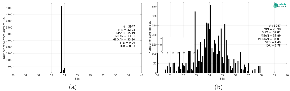
Figure 3: Histograms of SSS from Surface drifters (a) and SMAP SSS L2 v5.0 (JPL) (b) considering all match-up pairs per bins of 0.1 over the South Atlantic Ocean Pi-MEP region and for the full satellite product period.
