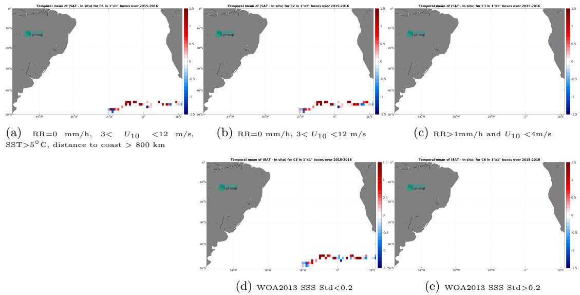
Figure 13: Temporal mean gridded over spatial boxes of size 1^\circ \times 1^\circ of \Delta SSS (SMAP SSS L2 v5.0 (JPL) - Surface drifters) for 5 different subdatasets corresponding to:RR=0 mm/h, 3 < U_{10} < 12 m/s, SST >5^\circ\text{C} , distance to coast > 800 km (a), RR=0 mm/h, 3 < U_{10} < 12 m/s (b), RR >1 mm/h and U_{10} < 4 m/s (c), WOA2013 SSS Std <0.2 (d), WOA2013 SSS Std >0.2 (e).
