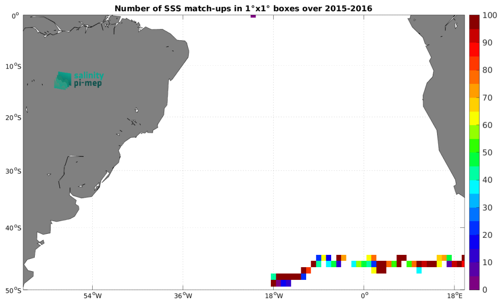
Figure 4: Number of SSS match-ups between Surface drifters SSS and the SMAP SSS L2 v5.0 (JPL) SSS product for the South Atlantic Ocean Pi-MEP region over 1^\circ \times 1^\circ boxes and for the full satellite product period.
