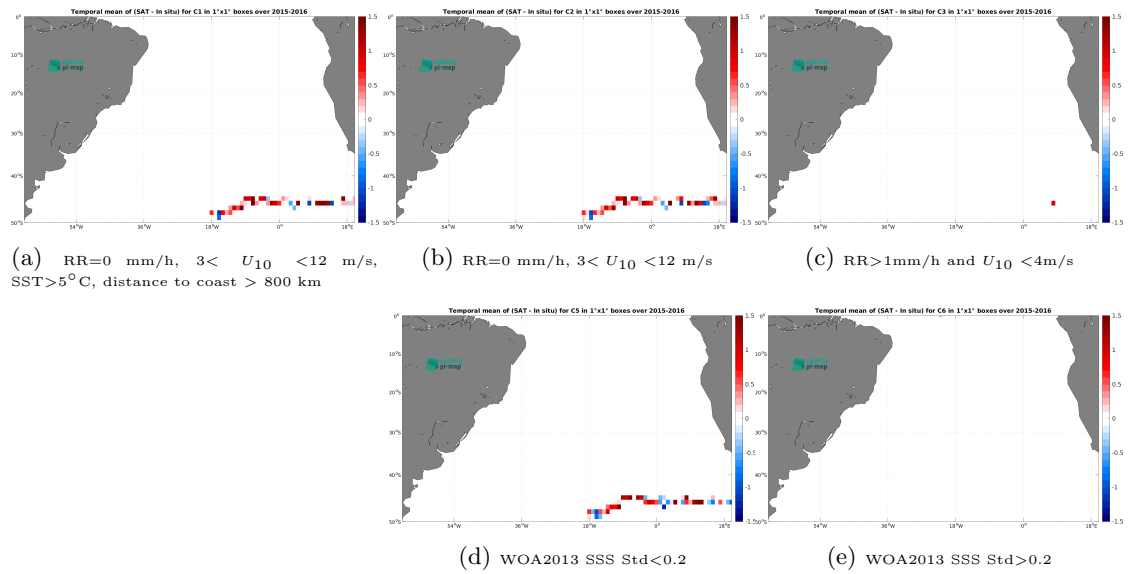
Figure 11: Temporal mean gridded over spatial boxes of size 1^\circ \times 1^\circ of \Delta SSS (SMAP SSS L2 v5.0 (JPL) - Surface drifters) for 5 different subdatasets corresponding to:RR=0 mm/h, 3 < U_{10} < 12 m/s, SST >5^\circ\text{C} , distance to coast > 800 km (a), RR=0 mm/h, 3 < U_{10} < 12 m/s (b), RR >1 mm/h and U_{10} < 4 m/s (c), WOA2013 SSS Std <0.2 (d), WOA2013 SSS Std >0.2 (e).
