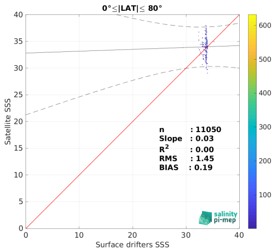
(a) 0^\circ \leq |LAT| \leq 80^\circ
