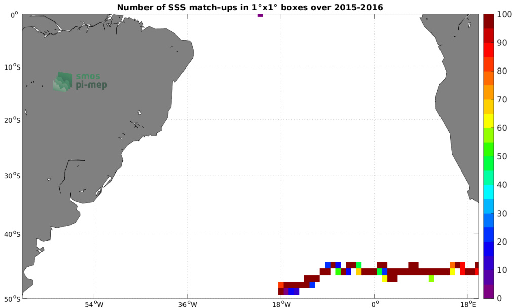
Figure 3: Number of SSS match-ups between Surface drifters SSS and the SMAP SSS L2 v5.0 (JPL) SSS product for the South Atlantic Ocean Pi-MEP region over 1^\circ \times 1^\circ boxes and for the full satellite product period.
