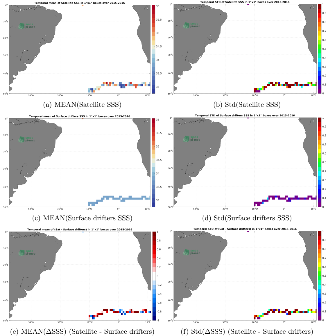
Figure 5: Temporal mean (left) and Std (right) of SSS from SMAP SSS L2 v5.0 (JPL) (top), Surface drifters (middle), and of \Delta SSS (Satellite - Surface drifters). Only match-up pairs are used to generate these maps.
