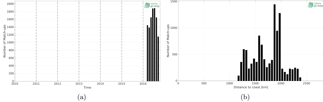
Figure 1: Number of match-ups between Surface drifters and SMAP SSS L2 v5.0 (JPL) SSS as a function of time (a) and as function of the distance to coast (b) over the South Atlantic Ocean Pi-MEP region and for the full satellite product period.
