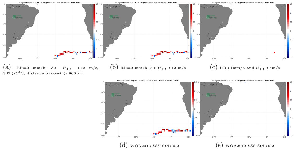
Figure 11: Temporal mean gridded over spatial boxes of size 1^{\circ}\times 1^{\circ} of \Delta\text{SSS} (SMAP SSS L2 v5.0 (JPL) - Surface drifters) for 5 different subdatasets corresponding to:RR=0 mm/h, 3 < U_{10} < 12 m/s, SST >5^{\circ}\text{C} , distance to coast > 800 km (a), RR=0 mm/h, 3 < U_{10} < 12 m/s (b), RR >1 mm/h and U_{10} < 4 m/s (c), WOA2013 SSS Std <0.2 (d), WOA2013 SSS Std >0.2 (e).
