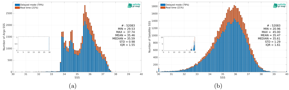
Figure 3: Histograms of SSS from Argo (a) and SMAP SSS L2 v5.0 (JPL) (b) considering all match-up pairs per bins of 0.1 over the South Atlantic Ocean Pi-MEP region and for the full satellite product period.
