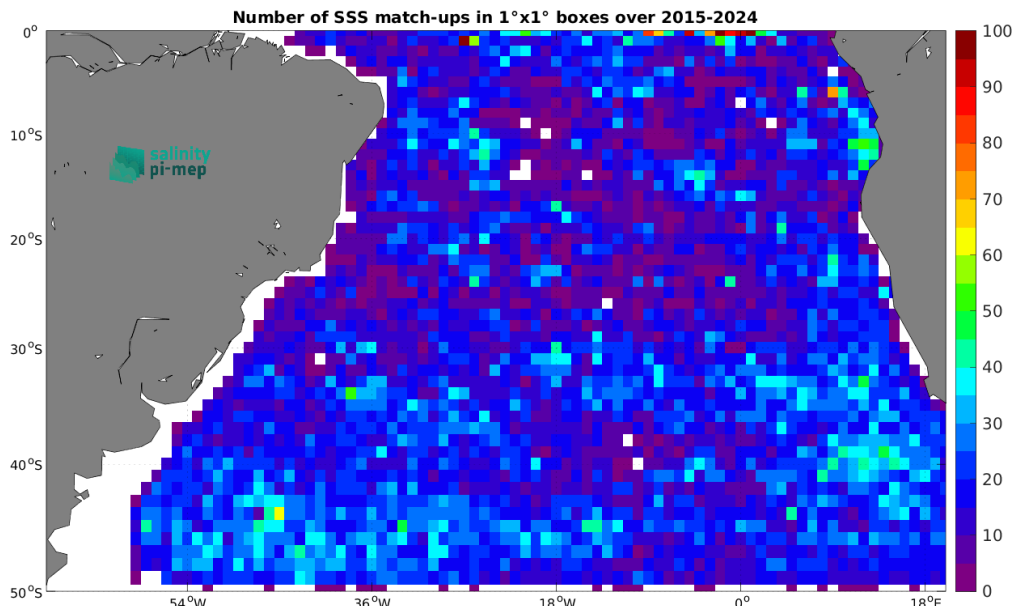
Figure 5: Number of SSS match-ups between Argo SSS and the SMAP SSS L2 v5.0 (JPL) SSS product for the South Atlantic Ocean Pi-MEP region over 1^\circ \times 1^\circ boxes and for the full satellite product period.
