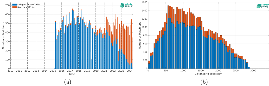
Figure 2: Number of match-ups between Argo and SMAP SSS L2 v5.0 (JPL) SSS as a function of time (a) and as function of the distance to coast (b) over the South Atlantic Ocean Pi-MEP region and for the full satellite product period.
