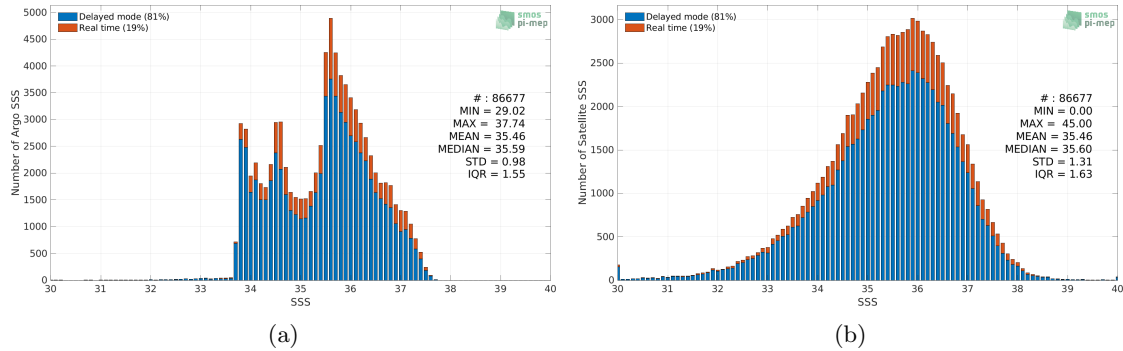
Figure 2: Histograms of SSS from Argo (a) and SMAP SSS L2 v5.0 (JPL) (b) considering all match-up pairs per bins of 0.1 over the South Atlantic Ocean Pi-MEP region and for the full satellite product period.
