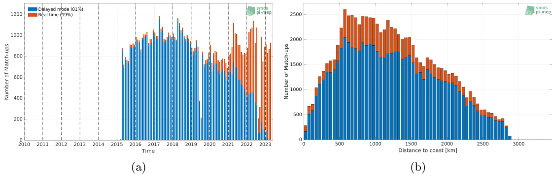
Figure 1: Number of match-ups between Argo and SMAP SSS L2 v5.0 (JPL) SSS as a function of time (a) and as function of the distance to coast (b) over the South Atlantic Ocean Pi-MEP region and for the full satellite product period.
