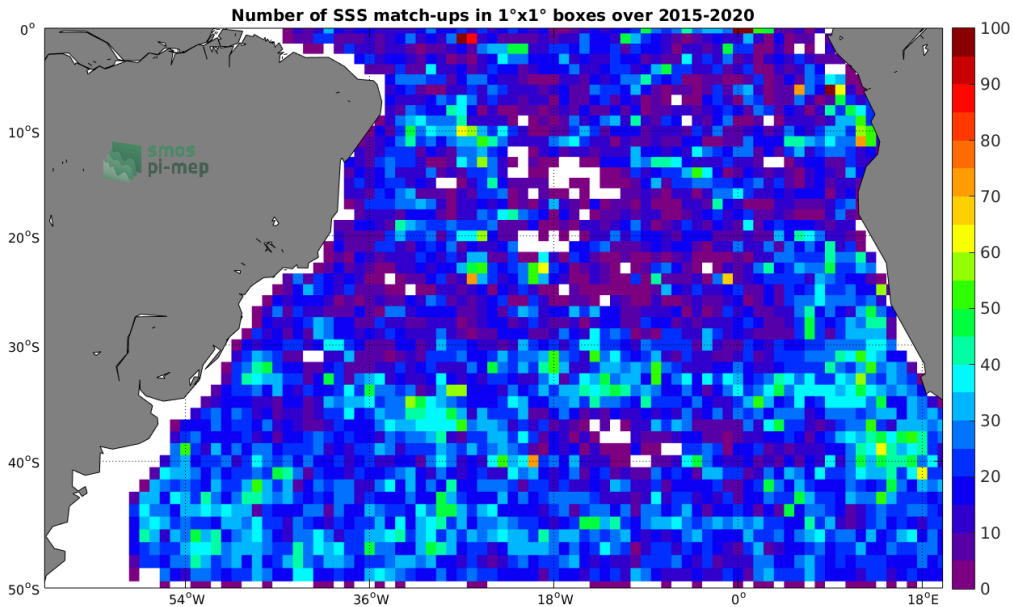
Figure 4: Number of SSS match-ups between Argo SSS and the SMAP SSS L2 v5.0 (JPL) SSS product for the South Atlantic Ocean Pi-MEP region over 1°x1° boxes and for the full satellite product period.
