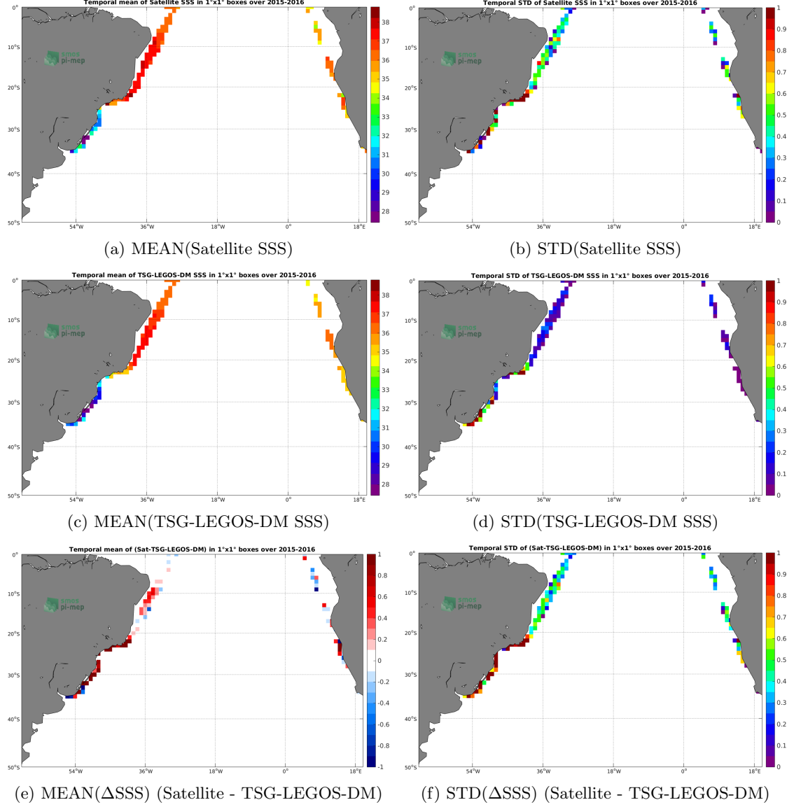
Figure 6: Temporal mean (left) and STD (right) of SSS from SMAP-L2-JPL-V4 (top), TSG-LEGOS-DM (middle), and of \Delta\text{SSS} (Satellite - TSG-LEGOS-DM). Only match-up pairs are used to generate these maps.
