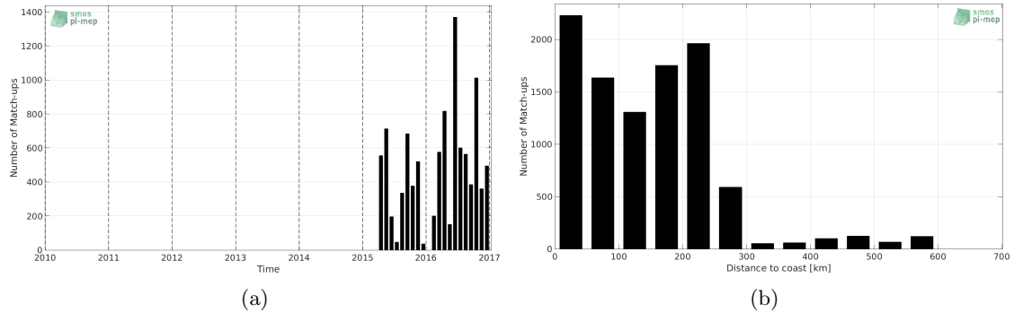
Figure 1: Number of match-ups between TSG-LEGOS-DM and SMAP-L2-JPL-V4 SSS as a function of time (a) and as function of the distance to coast (b) over the South Atlantic Ocean Pi-MEP region and for the full satellite product period.
