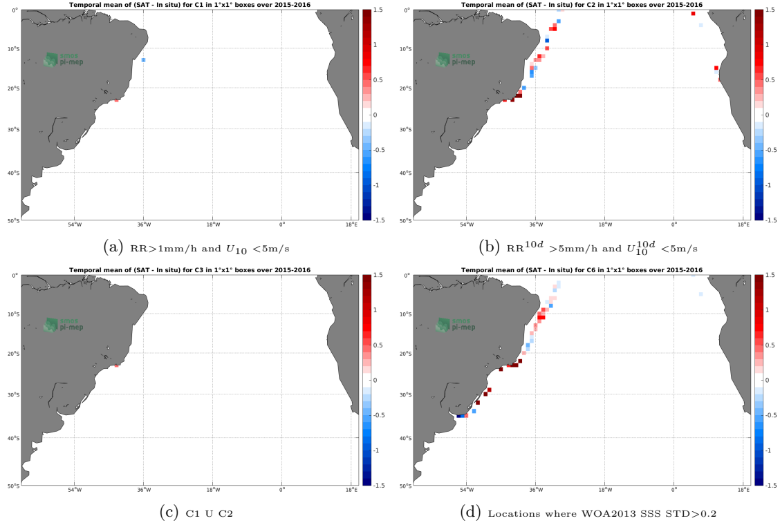
Figure 12: Temporal mean gridded over spatial boxes of size 1^\circ \times 1^\circ of \Delta SSS (SMAP-L2-JPL-V4 - TSG-LEGOS-DM) for 4 different subdatasets corresponding to: RR > 1\text{mm/h} and U_{10} < 5\text{m/s} (a), RR^{10d} > 5\text{mm/h} and U_{10}^{10d} < 5\text{m/s} (b), C1 U C2 (c), Locations where WOA2013 SSS STD > 0.2 (d).
