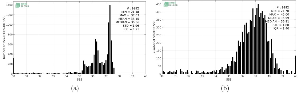
Figure 2: Histograms of SSS from TSG-LEGOS-DM (a) and SMAP-L2-JPL-V4 (b) considering all match-up pairs per bins of 0.1 over the South Atlantic Ocean Pi-MEP region and for the full satellite product period.
