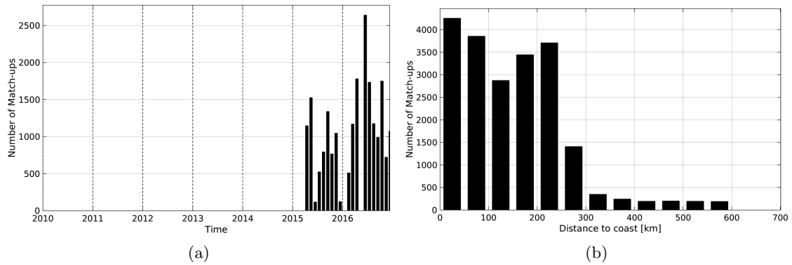
Figure 1: Number of match-ups between TSG-LEGOS-DM and SMAP-L2-JPL-V4 SSS as a function of time (a) and as function of the distance to coast (b) over the South Atlantic Ocean Pi-MEP region and for the full satellite product period.
