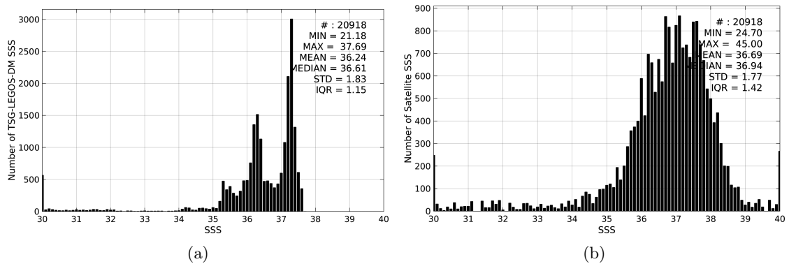
Figure 2: Histograms of SSS from TSG-LEGOS-DM (a) and SMAP-L2-JPL-V4 (b) considering all match-up pairs per bins of 0.1 over the South Atlantic Ocean Pi-MEP region and for the full satellite product period.
