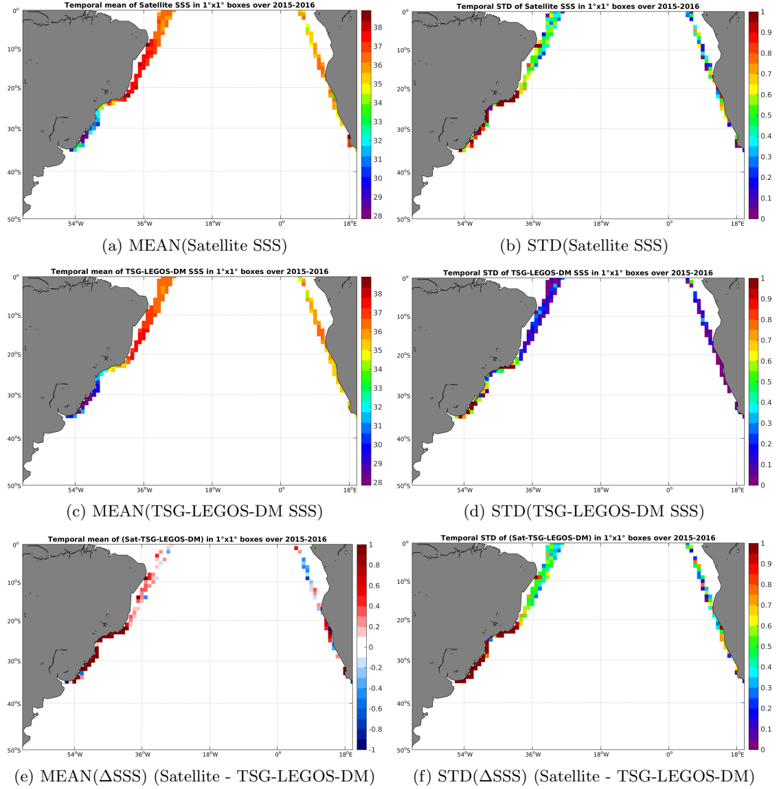
Figure 6: Temporal mean (left) and STD (right) of SSS from SMAP-L2-JPL-V4 (top), TSG-LEGOS-DM (middle), and of \Delta SSS (Satellite - TSG-LEGOS-DM). Only match-up pairs are used to generate these maps.
