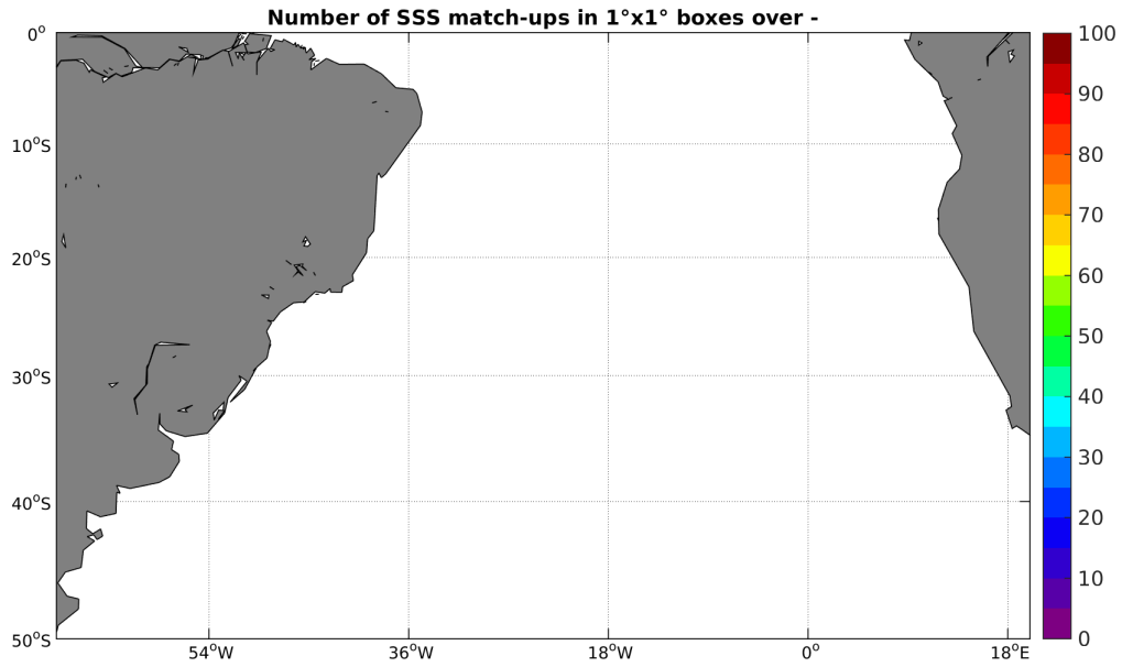
Figure 4: Number of SSS match-ups between TSG-GOSUD-Sailing-ship SSS and the SMAP-L2-JPL-V4 SSS product for the South Atlantic Ocean Pi-MEP region over 1^\circ \times 1^\circ boxes and for the full satellite product period.
