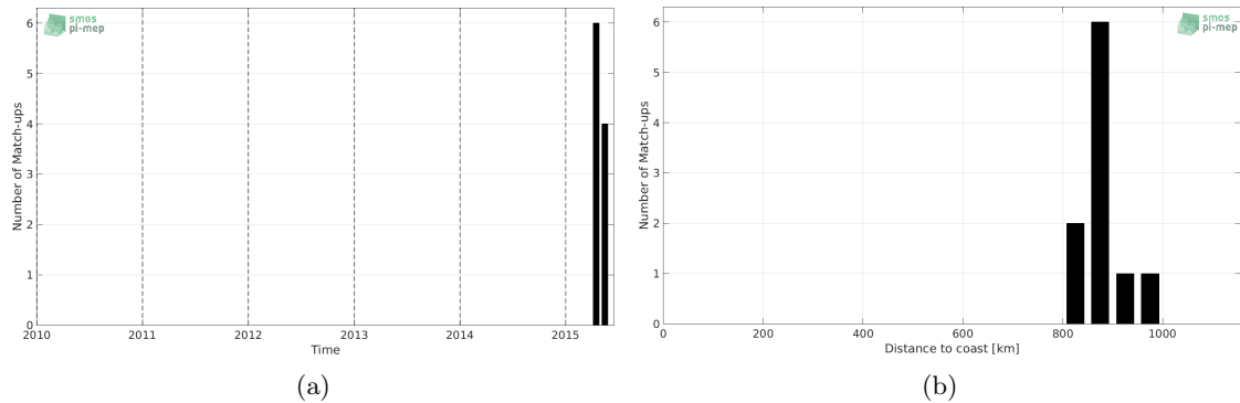
Figure 1: Number of match-ups between Sea mammals and SMAP-L2-JPL-V4 SSS as a function of time (a) and as function of the distance to coast (b) over the South Atlantic Ocean Pi-MEP region and for the full satellite product period.
