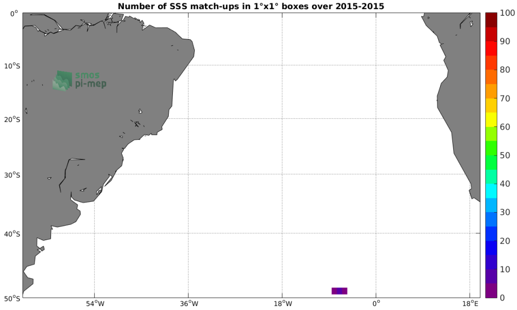
Figure 4: Number of SSS match-ups between Sea mammals SSS and the SMAP-L2-JPL-V4 SSS product for the South Atlantic Ocean Pi-MEP region over 1^\circ \times 1^\circ boxes and for the full satellite product period.
