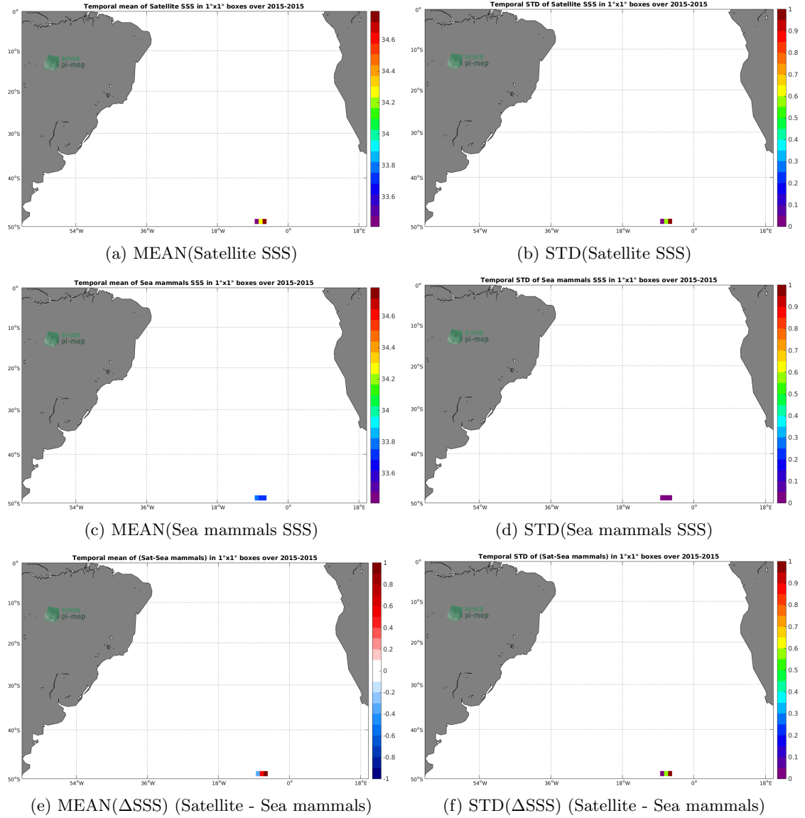
Figure 6: Temporal mean (left) and STD (right) of SSS from SMAP-L2-JPL-V4 (top), Sea mammals (middle), and of \Delta\text{SSS} (Satellite - Sea mammals). Only match-up pairs are used to generate these maps.
