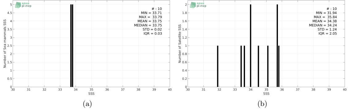
Figure 2: Histograms of SSS from Sea mammals (a) and SMAP-L2-JPL-V4 (b) considering all match-up pairs per bins of 0.1 over the South Atlantic Ocean Pi-MEP region and for the full satellite product period.
