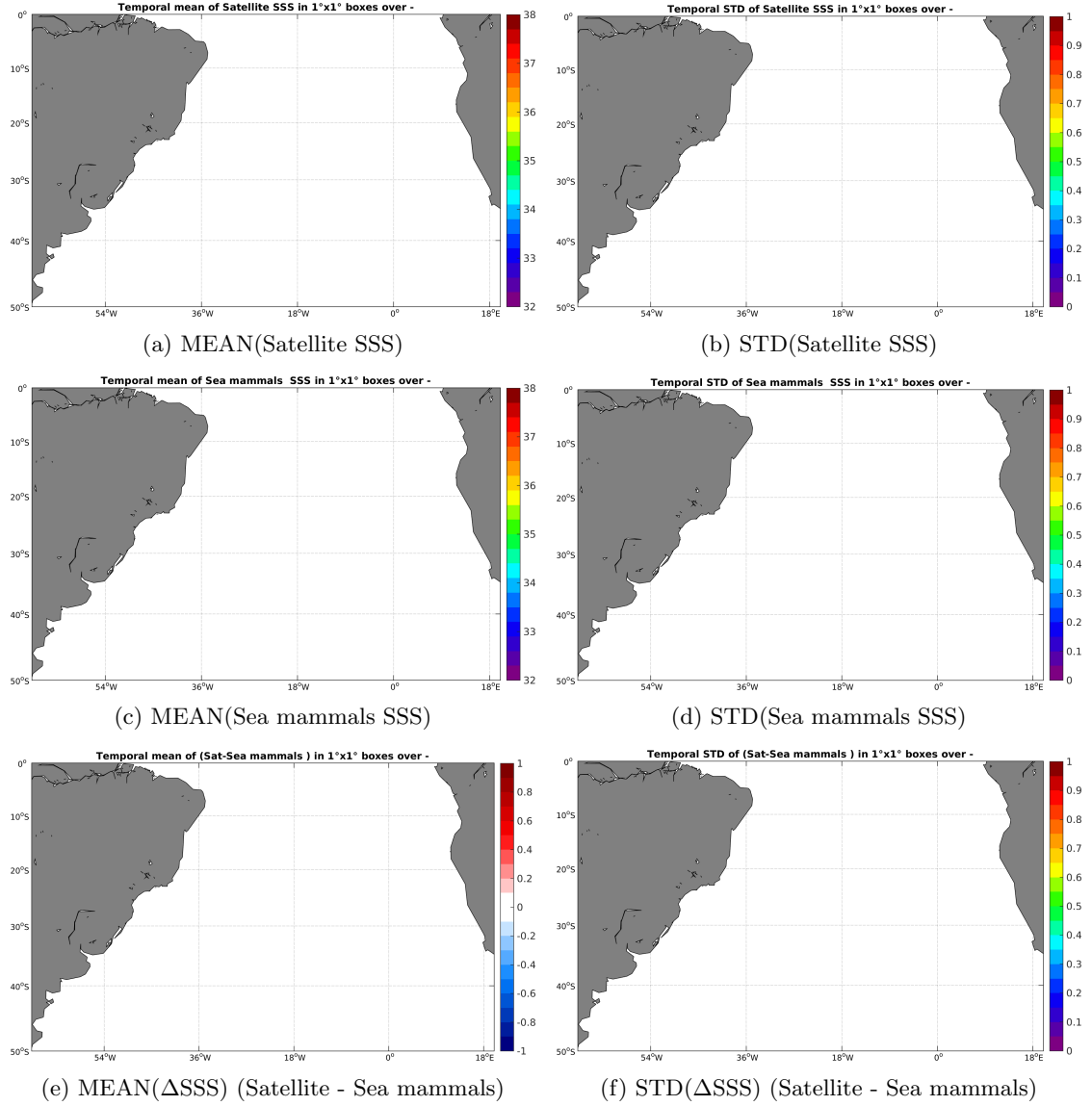
Figure 6: Temporal mean (left) and STD (right) of SSS from SMAP-L2-JPL-V4 (top), Sea mammals (middle), and of \Delta SSS (Satellite - Sea mammals). Only match-up pairs are used to generate these maps.
