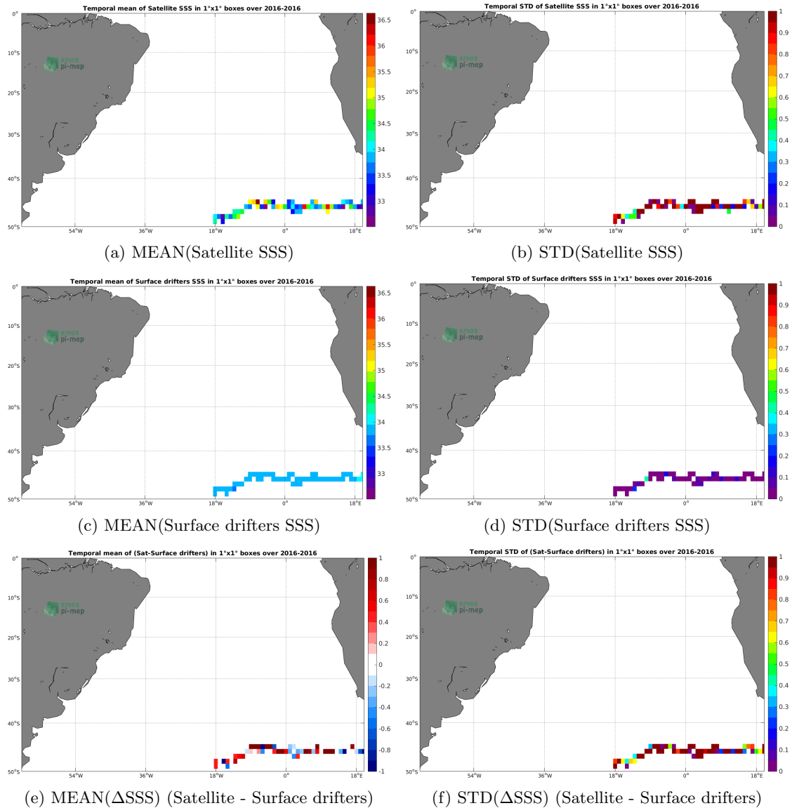
Figure 5: Temporal mean (left) and STD (right) of SSS from SMAP-L2-JPL-V4 (top), Surface drifters (middle), and of \Delta SSS (Satellite - Surface drifters). Only match-up pairs are used to generate these maps.
