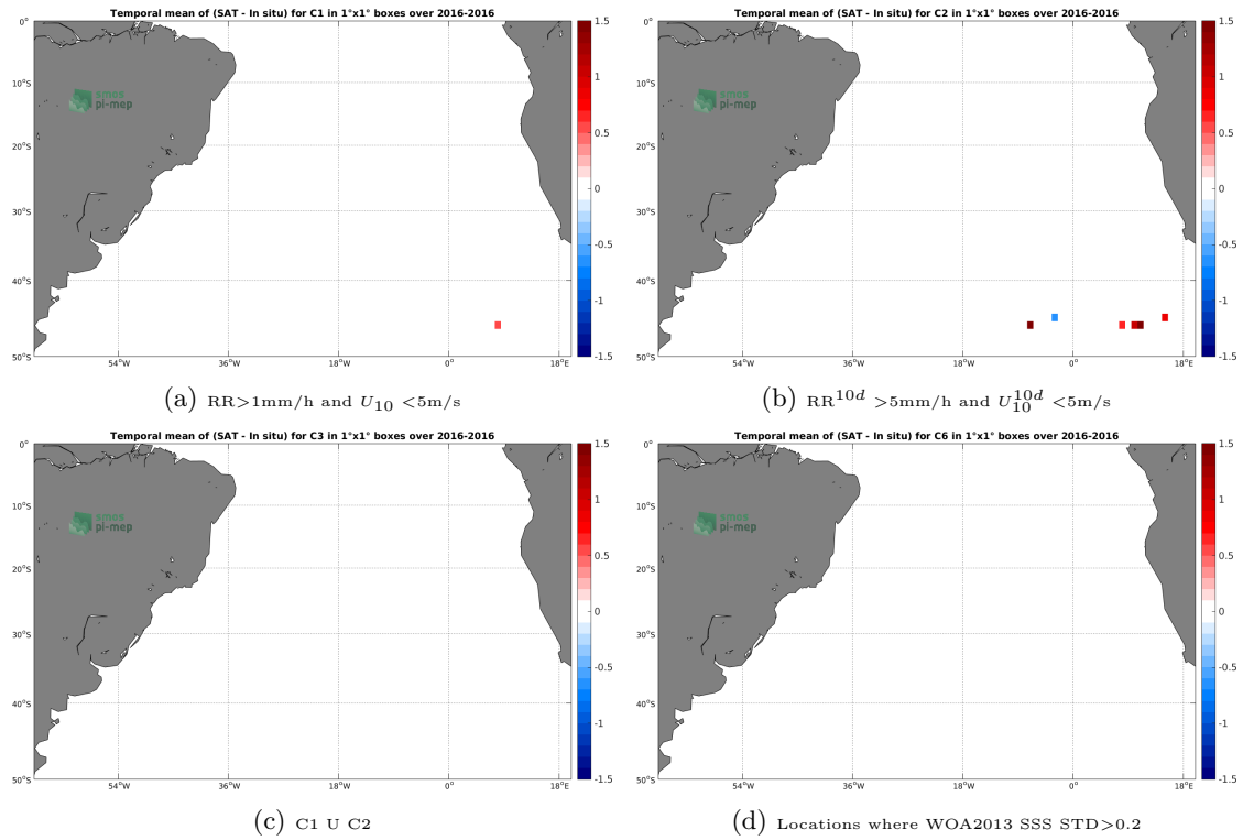
Figure 11: Temporal mean gridded over spatial boxes of size 1^\circ \times 1^\circ of \Delta SSS (SMAP-L2-JPL-V4 - Surface drifters) for 4 different subdatasets corresponding to: RR > 1mm/h and U_{10} < 5\text{m/s} (a), RR^{10d} > 5\text{mm/h} and U_{10}^{10d} < 5\text{m/s} (b), C1 U C2 (c), Locations where WOA2013 SSS STD > 0.2 (d).
