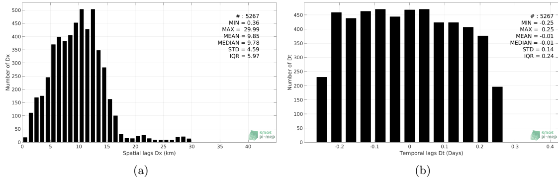
Figure 4: Histograms of the spatial (a) and temporal (b) lags between the time of the Surface drifters measurements and the date of the corresponding SMAP-L2-JPL-V4 SSS product.
