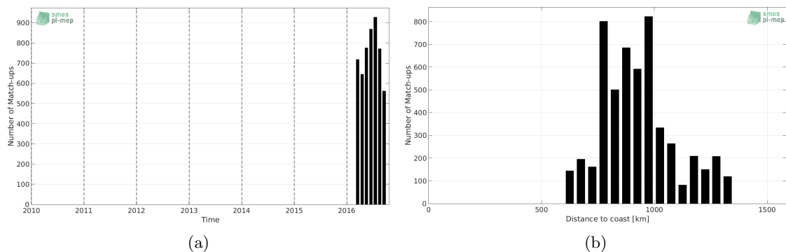
Figure 1: Number of match-ups between Surface drifters and SMAP-L2-JPL-V4 SSS as a function of time (a) and as function of the distance to coast (b) over the South Atlantic Ocean Pi-MEP region and for the full satellite product period.
