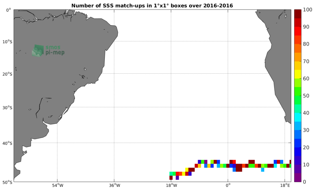
Figure 3: Number of SSS match-ups between Surface drifters SSS and the SMAP-L2-JPL-V4 SSS product for the South Atlantic Ocean Pi-MEP region over 1^\circ \times 1^\circ boxes and for the full satellite product period.
