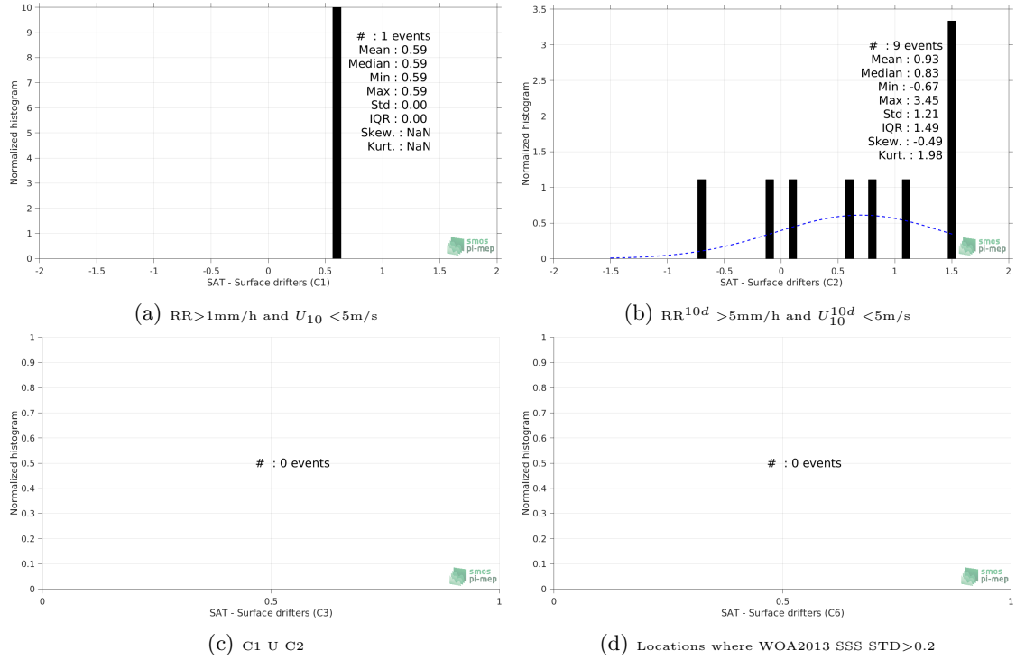
Figure 12: Normalized histogram of \Delta\text{SSS} (SMAP-L2-JPL-V4 - Surface drifters) for 6 different subdatasets corresponding to: RR > 1\text{mm/h} and U_{10} < 5\text{m/s} (a), RR^{10d} > 5\text{mm/h} and U_{10}^{10d} < 5\text{m/s} (b), C1 \cup C2 (c), Locations where WOA2013 SSS STD > 0.2 (d).
