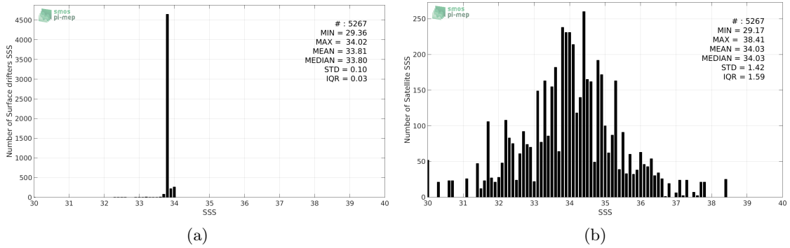
Figure 2: Histograms of SSS from Surface drifters (a) and SMAP-L2-JPL-V4 (b) considering all match-up pairs per bins of 0.1 over the South Atlantic Ocean Pi-MEP region and for the full satellite product period.
