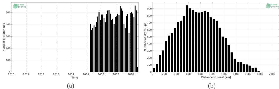
Figure 1: Number of match-ups between Argo and SMAP-L2-JPL-V4 SSS as a function of time (a) and as function of the distance to coast (b) over the South Atlantic Ocean Pi-MEP region and for the full satellite product period.
