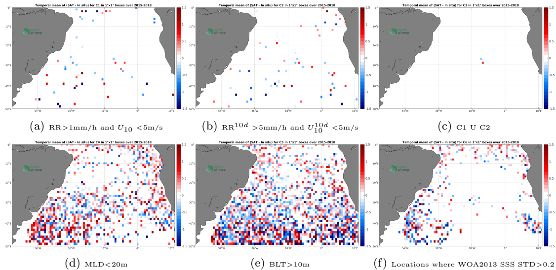
Figure 12: Temporal mean gridded over spatial boxes of size 1^\circ \times 1^\circ of \Delta\text{SSS} (SMAP-L2-JPL-V4 - Argo) for 6 different subdatasets corresponding to: RR > 1\text{mm/h} and U_{10} < 5\text{m/s} (a), RR^{10d} > 5\text{mm/h} and U_{10}^{10d} < 5\text{m/s} (b), C1 U C2 (c), MLD < 20\text{m} (d), BLT > 10\text{m} (e), Locations where WOA2013 SSS STD > 0.2 (f).
