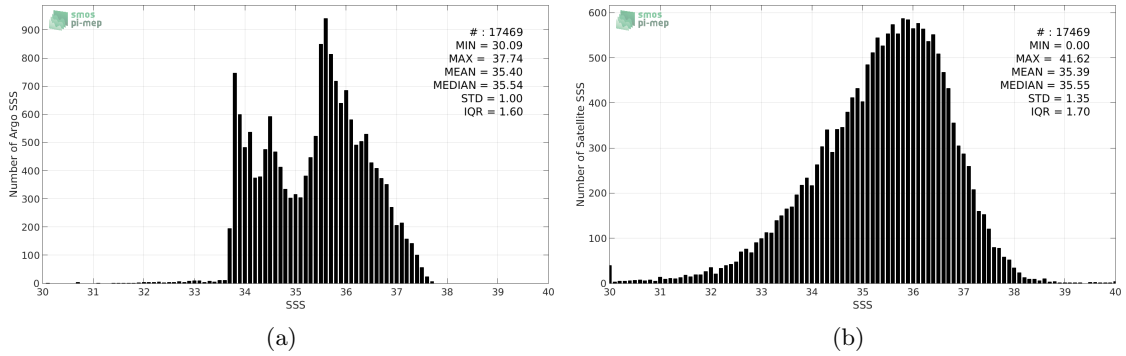
Figure 2: Histograms of SSS from Argo (a) and SMAP-L2-JPL-V4 (b) considering all match-up pairs per bins of 0.1 over the South Atlantic Ocean Pi-MEP region and for the full satellite product period.
