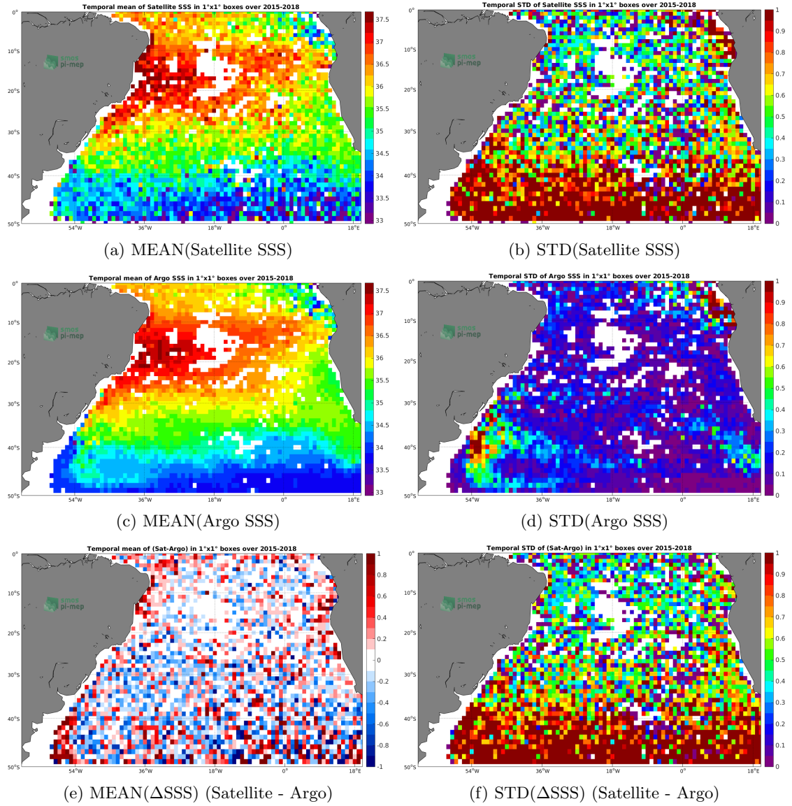
Figure 6: Temporal mean (left) and STD (right) of SSS from SMAP-L2-JPL-V4 (top), Argo (middle), and of \Delta\text{SSS} (Satellite - Argo). Only match-up pairs are used to generate these maps.
