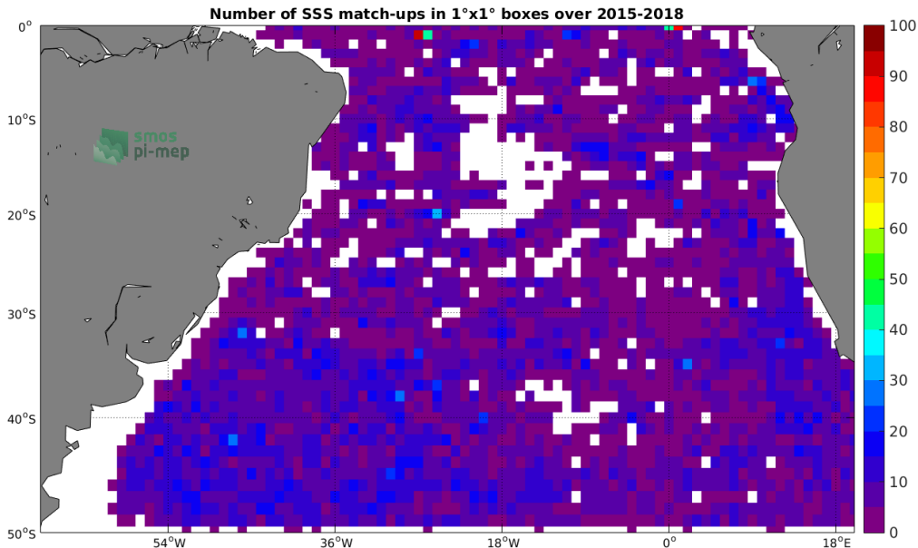
Figure 4: Number of SSS match-ups between Argo SSS and the SMAP-L2-JPL-V4 SSS product for the South Atlantic Ocean Pi-MEP region over 1^{\circ} \times 1^{\circ} boxes and for the full satellite product period.
