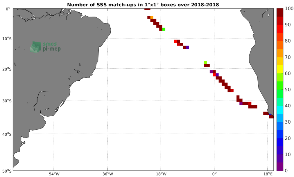
Figure 4: Number of SSS match-ups between TSG-SAMOS SSS and the SMAP-L2-JPL-V4.3 SSS product for the South Atlantic Ocean Pi-MEP region over 1^\circ \times 1^\circ boxes and for the full satellite product period.
