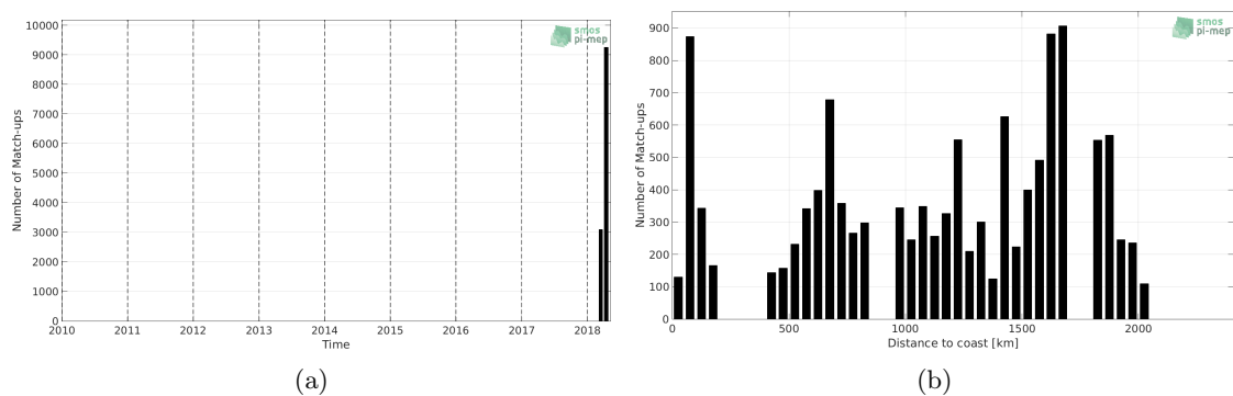
Figure 1: Number of match-ups between TSG-SAMOS and SMAP-L2-JPL-V4.3 SSS as a function of time (a) and as function of the distance to coast (b) over the South Atlantic Ocean Pi-MEP region and for the full satellite product period.
