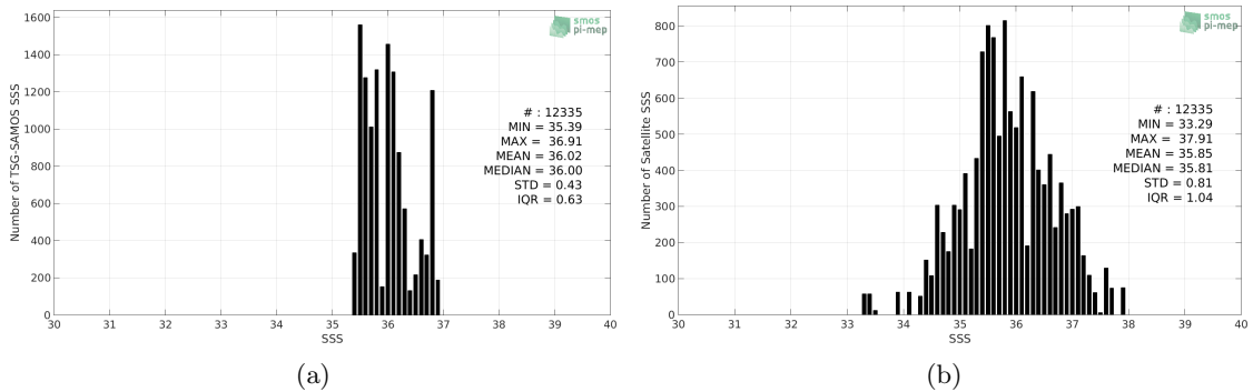
Figure 2: Histograms of SSS from TSG-SAMOS (a) and SMAP-L2-JPL-V4.3 (b) considering all match-up pairs per bins of 0.1 over the South Atlantic Ocean Pi-MEP region and for the full satellite product period.
