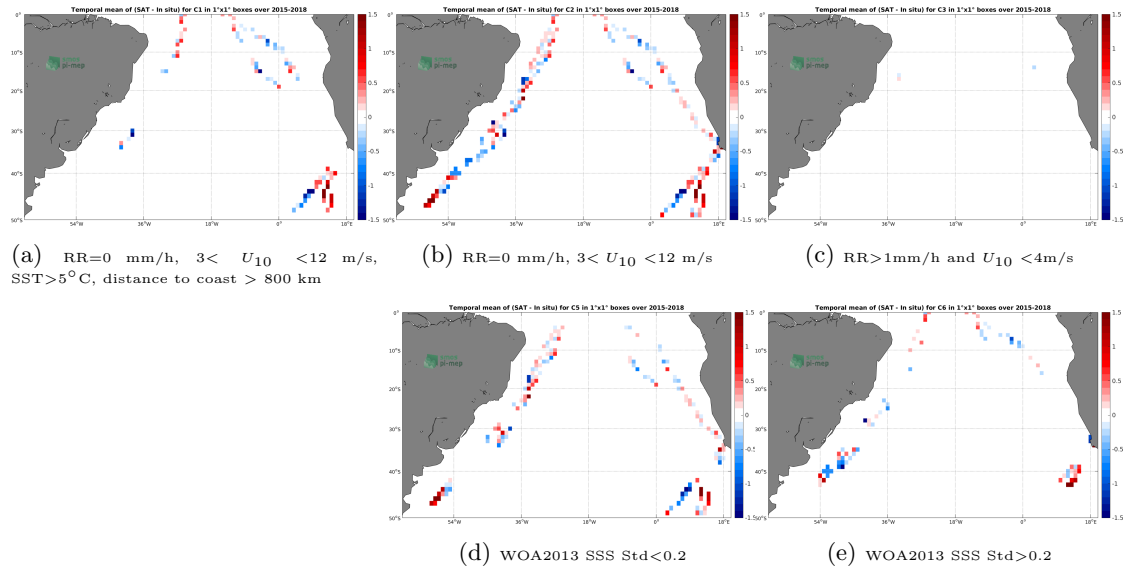
Figure 12: Temporal mean gridded over spatial boxes of size 1^\circ \times 1^\circ of \Delta SSS (SMAP-L2-JPL-V4.3 - TSG-POLARSTERN) for 5 different subdatasets corresponding to:RR=0 mm/h, 3 < U_{10} < 12 m/s, SST >5^\circ\text{C} , distance to coast > 800 km (a), RR=0 mm/h, 3 < U_{10} < 12 m/s (b), RR >1 mm/h and U_{10} < 4 m/s (c), WOA2013 SSS Std <0.2 (d), WOA2013 SSS Std >0.2 (e).
