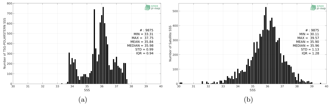
Figure 2: Histograms of SSS from TSG-POLARSTERN (a) and SMAP-L2-JPL-V4.3 (b) considering all match-up pairs per bins of 0.1 over the South Atlantic Ocean Pi-MEP region and for the full satellite product period.
