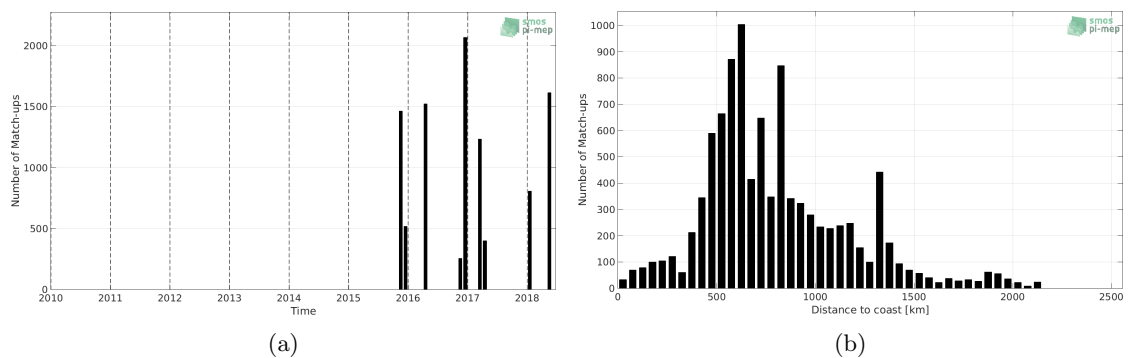
Figure 1: Number of match-ups between TSG-POLARSTERN and SMAP-L2-JPL-V4.3 SSS as a function of time (a) and as function of the distance to coast (b) over the South Atlantic Ocean Pi-MEP region and for the full satellite product period.
