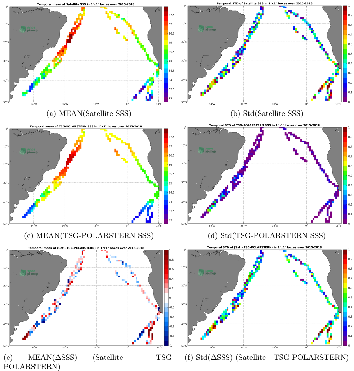
Figure 6: Temporal mean (left) and Std (right) of SSS from SMAP-L2-JPL-V4.3 (top), TSG-POLARSTERN (middle), and of \Delta SSS (Satellite - TSG-POLARSTERN). Only match-up pairs are used to generate these maps.
