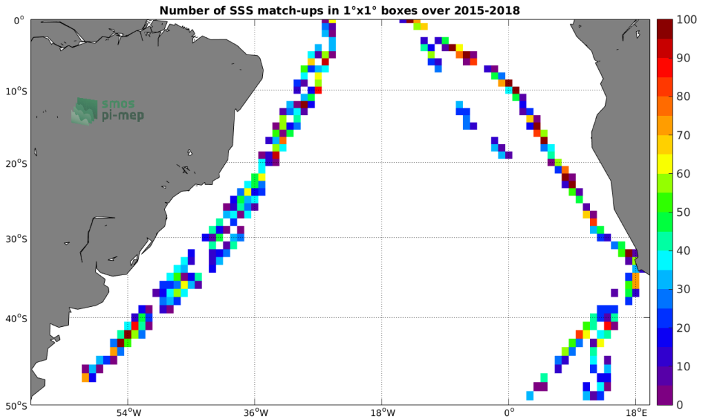
Figure 4: Number of SSS match-ups between TSG-POLARSTERN SSS and the SMAP-L2-JPL-V4.3 SSS product for the South Atlantic Ocean Pi-MEP region over 1^\circ \times 1^\circ boxes and for the full satellite product period.
