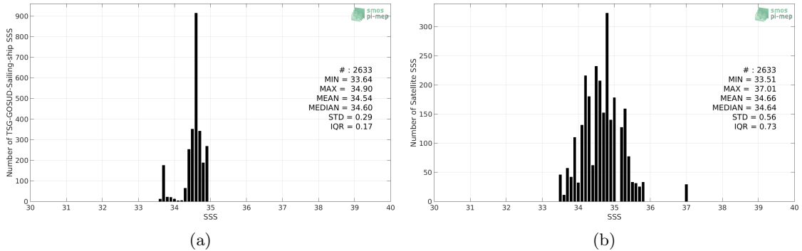
Figure 2: Histograms of SSS from TSG-GOSUD-Sailing-ship (a) and SMAP-L2-JPL-V4.3 (b) considering all match-up pairs per bins of 0.1 over the South Atlantic Ocean Pi-MEP region and for the full satellite product period.
