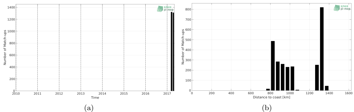
Figure 1: Number of match-ups between TSG-GOSUD-Sailing-ship and SMAP-L2-JPL-V4.3 SSS as a function of time (a) and as function of the distance to coast (b) over the South Atlantic Ocean Pi-MEP region and for the full satellite product period.
