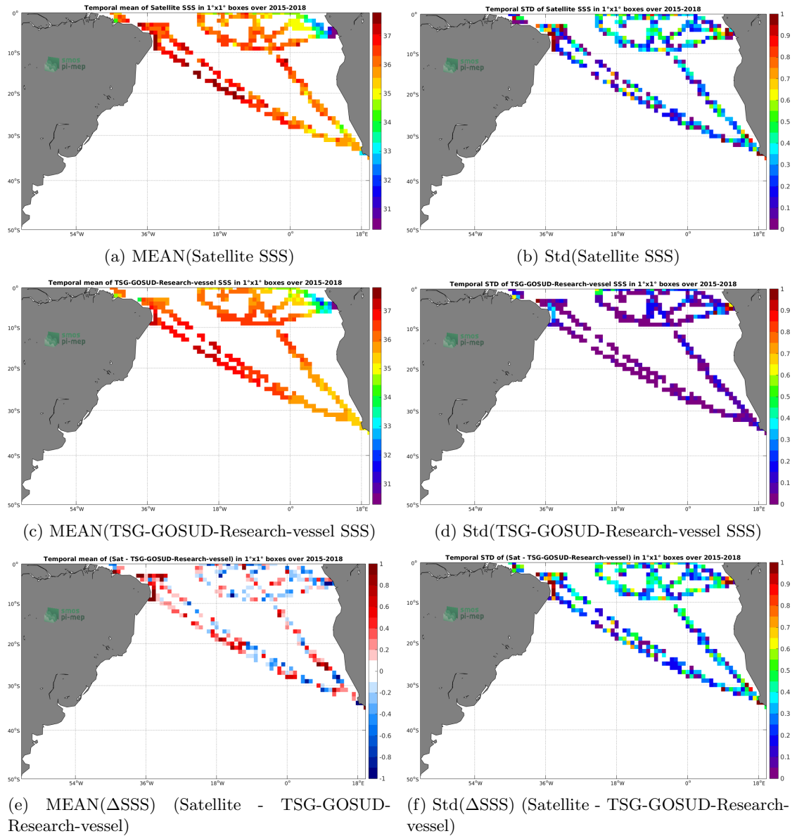
Figure 6: Temporal mean (left) and Std (right) of SSS from SMAP-L2-JPL-V4.3 (top), TSG-GOSUD-Research-vessel (middle), and of \Delta SSS (Satellite - TSG-GOSUD-Research-vessel). Only match-up pairs are used to generate these maps.
