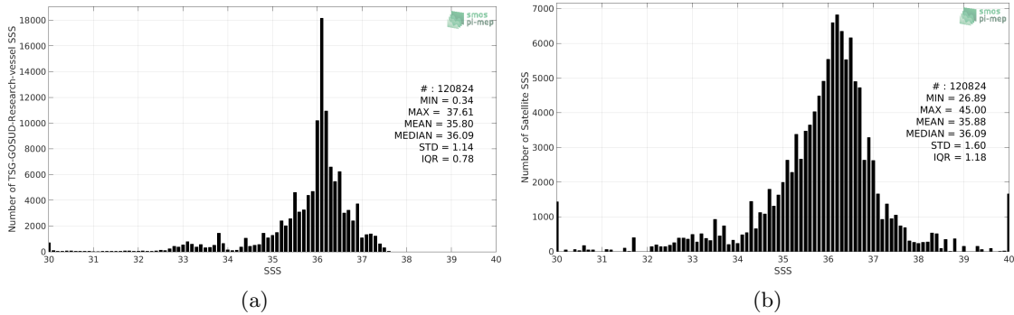
Figure 2: Histograms of SSS from TSG-GOSUD-Research-vessel (a) and SMAP-L2-JPL-V4.3 (b) considering all match-up pairs per bins of 0.1 over the South Atlantic Ocean Pi-MEP region and for the full satellite product period.
