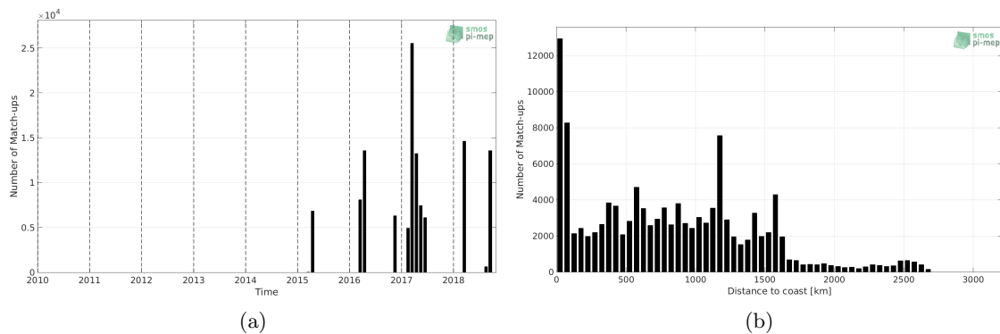
Figure 1: Number of match-ups between TSG-GOSUD-Research-vessel and SMAP-L2-JPL-V4.3 SSS as a function of time (a) and as function of the distance to coast (b) over the South Atlantic Ocean Pi-MEP region and for the full satellite product period.
