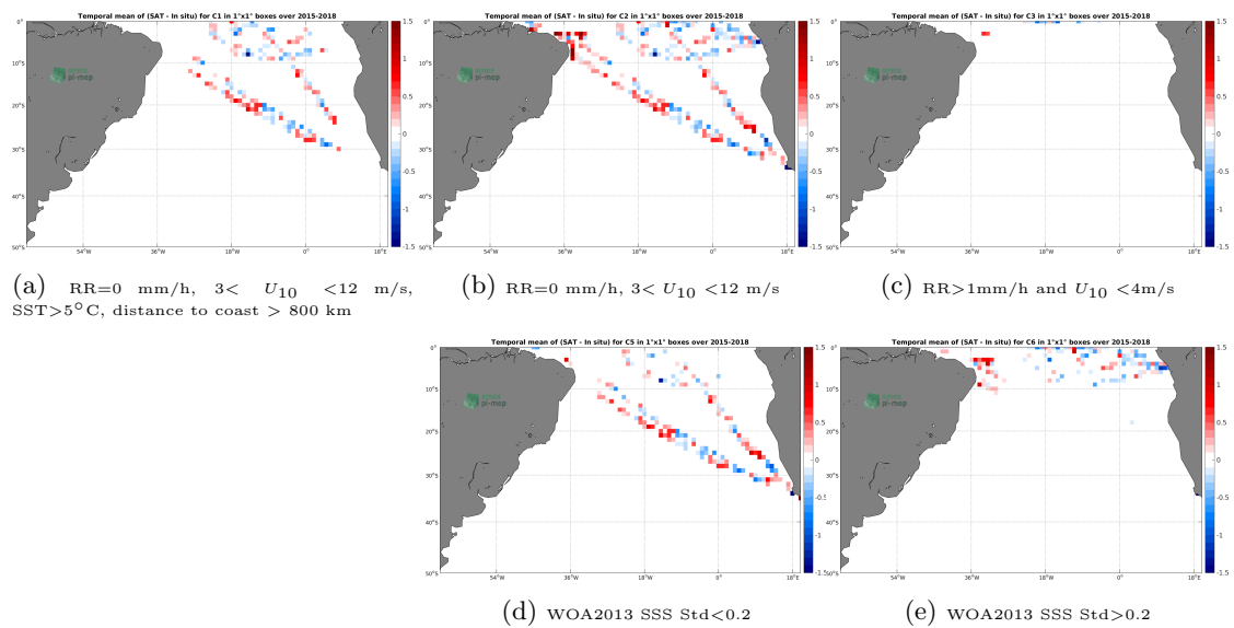
Figure 12: Temporal mean gridded over spatial boxes of size 1^\circ \times 1^\circ of \Delta SSS (SMAP-L2-JPL-V4.3 - TSG-GOSUD-Research-vessel) for 5 different subdatasets corresponding to:RR=0 mm/h, 3 < U_{10} < 12 m/s, SST>5°C, distance to coast > 800 km (a), RR=0 mm/h, 3 < U_{10} < 12 m/s (b), RR>1mm/h and U_{10} < 4 m/s (c), WOA2013 SSS Std<0.2 (d), WOA2013 SSS Std>0.2 (e).
