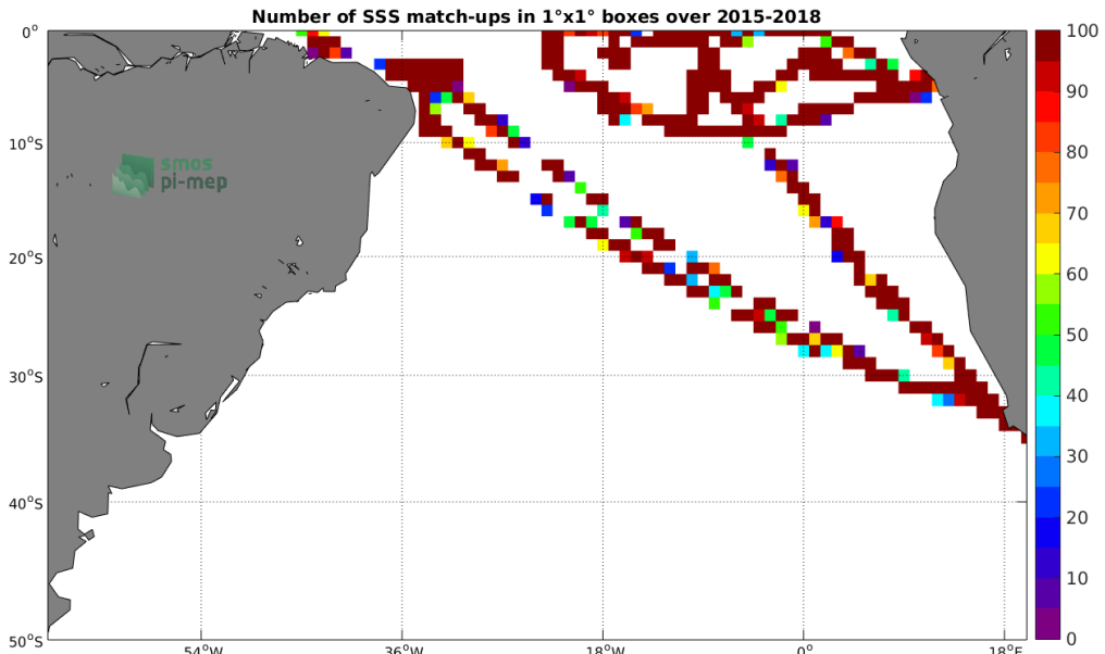
Figure 4: Number of SSS match-ups between TSG-GOSUD-Research-vessel SSS and the SMAP-L2-JPL-V4.3 SSS product for the South Atlantic Ocean Pi-MEP region over 1^\circ \times 1^\circ boxes and for the full satellite product period.
