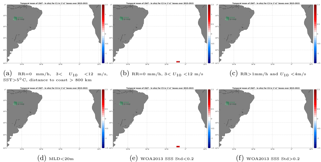
Figure 12: Temporal mean gridded over spatial boxes of size 1^{\circ}\times 1^{\circ} of \Delta\text{SSS} (SMAP-L2-JPL-V4.3 - Sea mammals) for 6 different subdatasets corresponding to:RR=0 mm/h, 3 < U_{10} < 12 m/s, SST >5^{\circ}\text{C} , distance to coast > 800 km (a), RR=0 mm/h, 3 < U_{10} < 12 m/s (b), RR >1 mm/h and U_{10} < 4 m/s (c),MLD <20 m (d),WOA2013 SSS Std <0.2 (e),WOA2013 SSS Std >0.2 (f).
