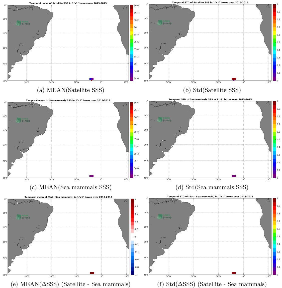
Figure 6: Temporal mean (left) and Std (right) of SSS from SMAP-L2-JPL-V4.3 (top), Sea mammals (middle), and of \Delta\text{SSS} (Satellite - Sea mammals). Only match-up pairs are used to generate these maps.
