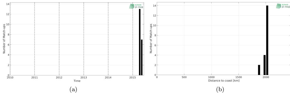
Figure 1: Number of match-ups between Sea mammals and SMAP-L2-JPL-V4.3 SSS as a function of time (a) and as function of the distance to coast (b) over the South Atlantic Ocean Pi-MEP region and for the full satellite product period.
