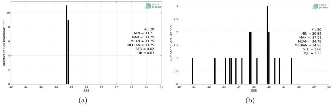
Figure 2: Histograms of SSS from Sea mammals (a) and SMAP-L2-JPL-V4.3 (b) considering all match-up pairs per bins of 0.1 over the South Atlantic Ocean Pi-MEP region and for the full satellite product period.
