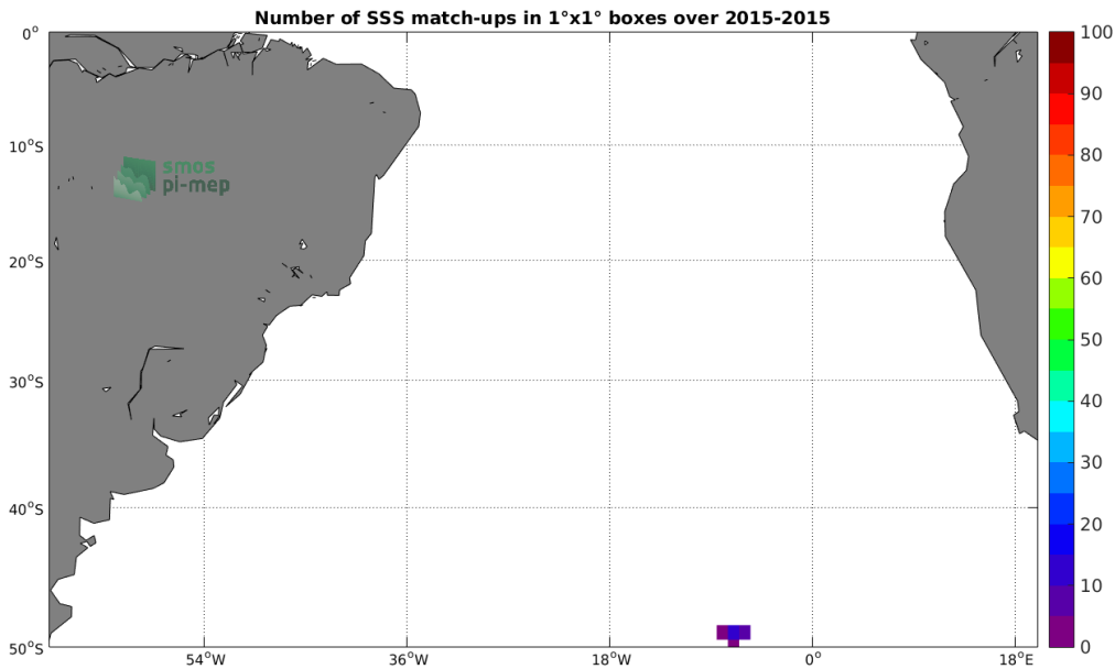
Figure 4: Number of SSS match-ups between Sea mammals SSS and the SMAP-L2-JPL-V4.3 SSS product for the South Atlantic Ocean Pi-MEP region over 1°x1° boxes and for the full satellite product period.
