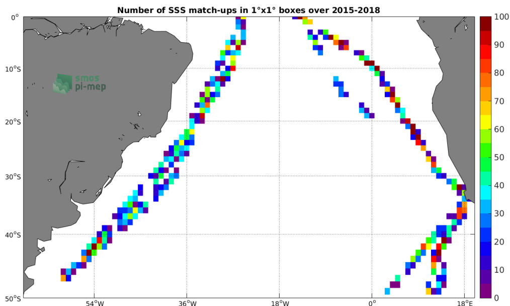
Figure 4: Number of SSS match-ups between TSG-POLARSTERN SSS and the SMAP-L2-JPL-V4.2 SSS product for the South Atlantic Ocean Pi-MEP region over 1^{\circ} \times 1^{\circ} boxes and for the full satellite product period.
