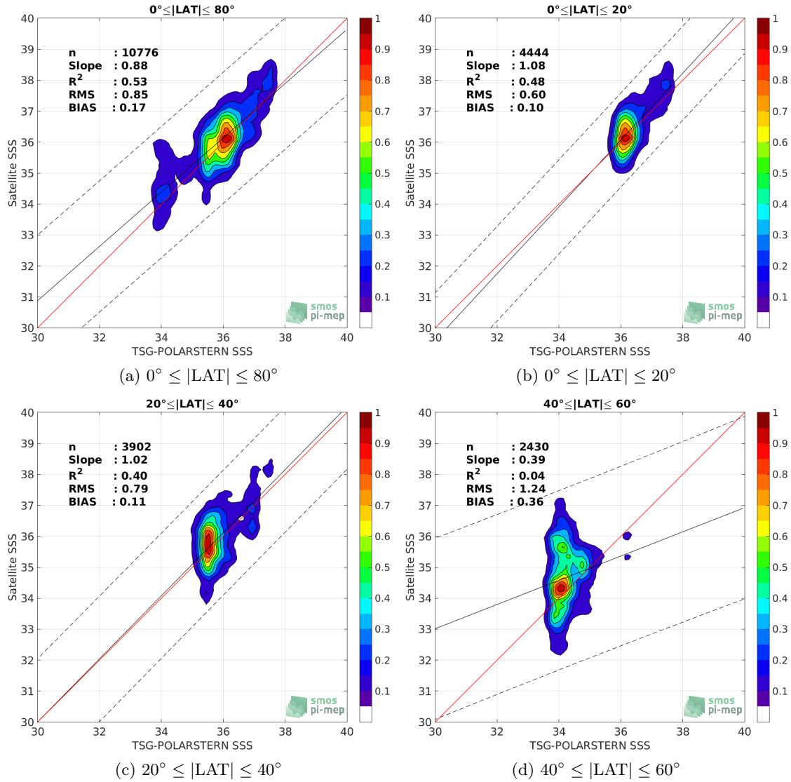
Figure 9: Contour maps of the concentration of SMAP-L2-JPL-V4.2 SSS (y-axis) versus TSG-POLARSTERN SSS (x-axis) at match-up pairs for different latitude bands. For each plot, the red line shows x=y . The black thin and dashed lines indicate a linear fit through the data cloud and the \pm 95\% confidence levels, respectively. The number match-up pairs n , the slope and R^2 coefficient of the linear fit, the root mean square (RMS) and the mean bias between satellite and in situ data are indicated for each latitude band in each plots.
