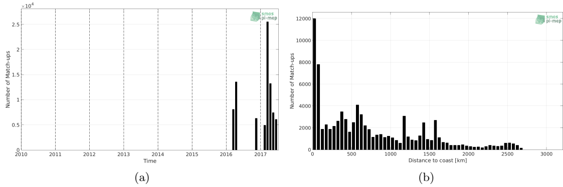
Figure 1: Number of match-ups between TSG-GOSUD-Research-vessel and SMAP-L2-JPL-V4.2 SSS as a function of time (a) and as function of the distance to coast (b) over the South Atlantic Ocean Pi-MEP region and for the full satellite product period.
