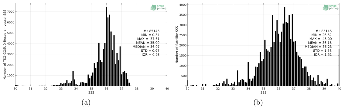
Figure 2: Histograms of SSS from TSG-GOSUD-Research-vessel (a) and SMAP-L2-JPL-V4.2 (b) considering all match-up pairs per bins of 0.1 over the South Atlantic Ocean Pi-MEP region and for the full satellite product period.
