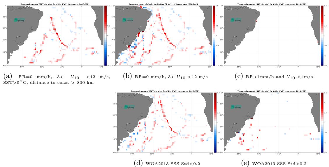
Figure 14: Temporal mean gridded over spatial boxes of size 1^\circ \times 1^\circ of \Delta SSS (ISAS v7 - Monthly (Ifremer-LOPS-CMEMS) - TSG (GOSUD-Sailing-ship)) for 5 different subdatasets corresponding to:RR=0 mm/h, 3 < U_{10} < 12 m/s, SST>5°C, distance to coast > 800 km (a), RR=0 mm/h, 3 < U_{10} < 12 m/s (b), RR>1mm/h and U_{10} < 4 m/s (c), WOA2013 SSS Std<0.2 (d), WOA2013 SSS Std>0.2 (e).
