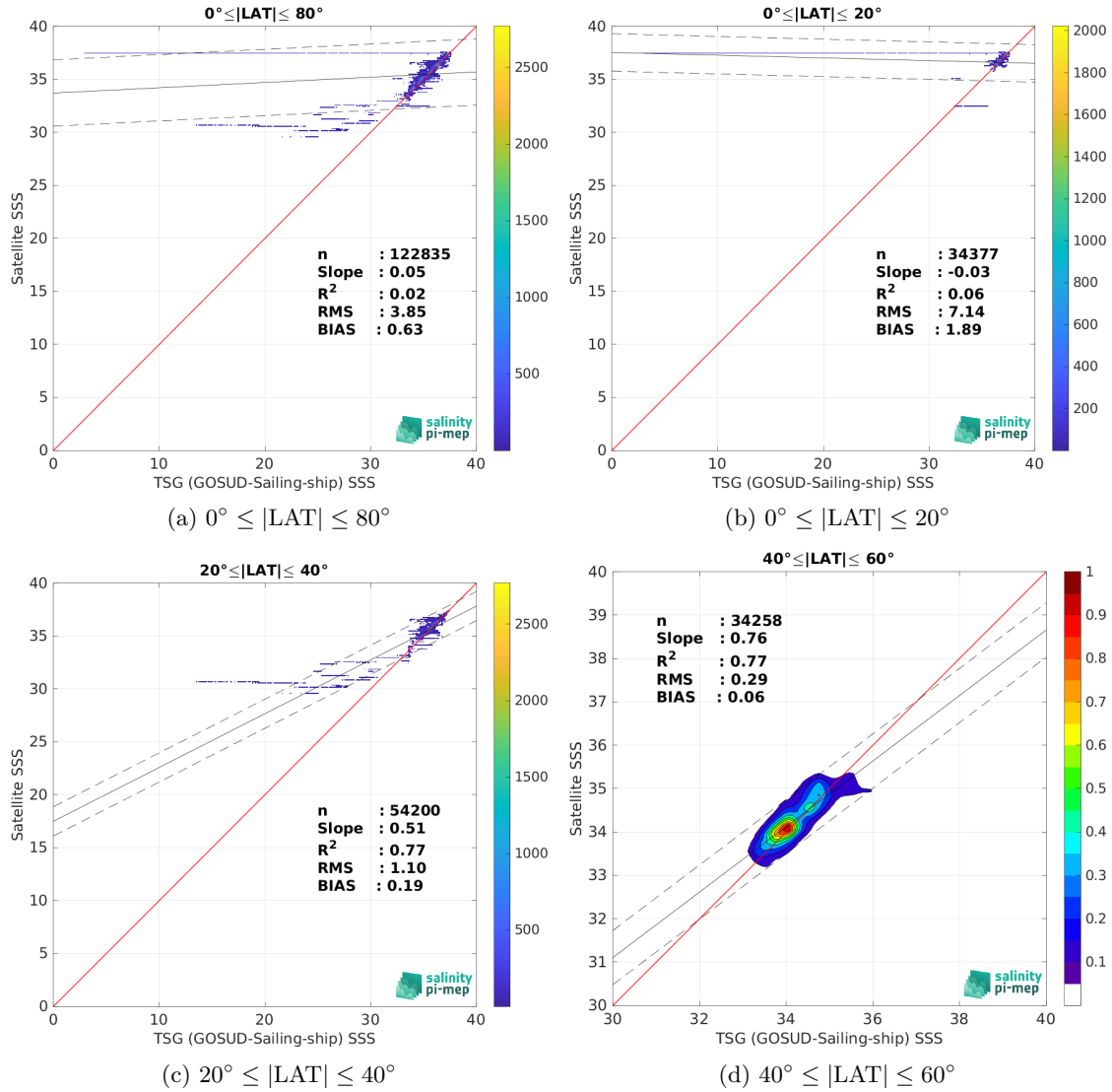
Figure 10: Contour maps of the concentration of ISAS v7 - Monthly (Ifremer-LOPS-CMEMS) SSS (y-axis) versus TSG (GOSUD-Sailing-ship) SSS (x-axis) at match-up pairs for different latitude bands. For each plot, the red line shows x=y . The black thin and dashed lines indicate a linear fit through the data cloud and the \pm 95\% confidence levels, respectively. The number match-up pairs n , the slope and R^2 coefficient of the linear fit, the root mean square (RMS) and the mean bias between satellite and in situ data are indicated for each latitude band in each plots.
